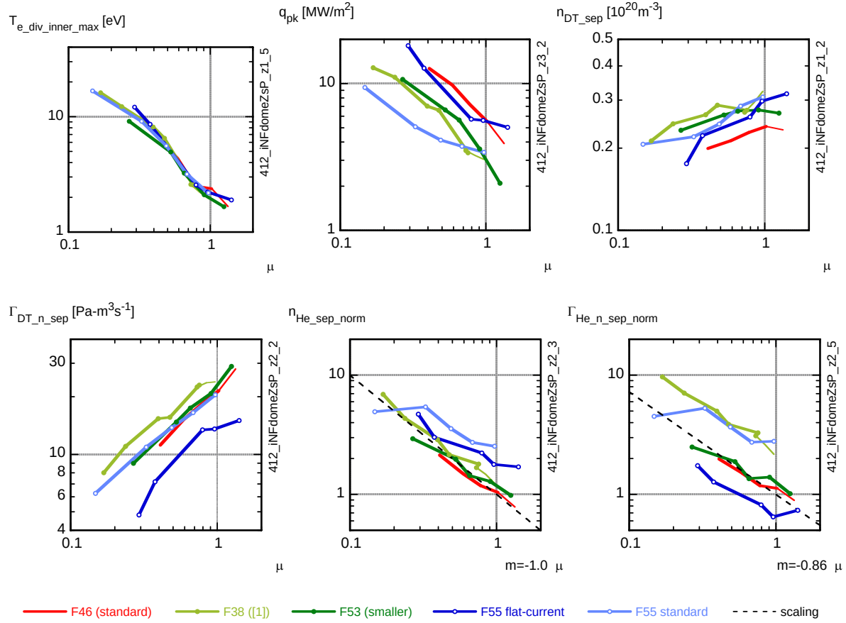
Fig. 2. Modelling results vs. normalized neutral pressure under the dome, \mu [3], for the divertor geometries considered: (a) maximum temperature at the inner divertor target (b) peak power loading of the targets; (c) average fuel ion density at the separatrix; (d) fuel neutral influx to the core; (e) average helium ion density at the separatrix; (f) helium neutral influx to the core. The helium data are normalized to the helium production rate and pumping speed [3]. Data for a previously studied variant F38 are added to show the progression.
