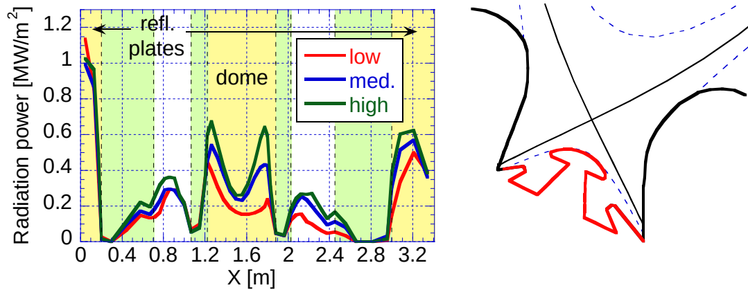
Fig. 3. Left: radiation power loads on the structures in PFR for the modified dome F53 for three operational points: at low density, intermediate, and near the high-density limit (full detachment) of the operational window. Right: Geometry layout for the evaluation of the radiation. The loads are given along the contour marked red, with x=0 at the inner divertor. The separatrix and the limits of the computational grid are also shown.
