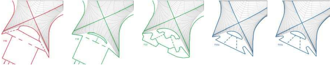
Fig. 1. Dome geometry, left to the right: F46 – the original reference geometry [2]; F38 – reduced dome used in [1]; F53 – smaller dome; F55 – shifted modified dome and inner target, flat current equilibrium I_i = 0.63 ; the same F55 with reference plasma equilibrium. Dashed lines show partially transparent structures giving access to the pump ducts.
