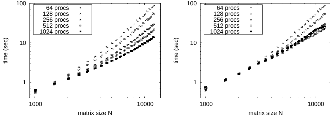
Figure 5: Run times computing ten percent of the eigenpairs of matrices with eigenvalues randomly generated in [0,1] , using PDSYEVX (left) and PDSYEV (right).
