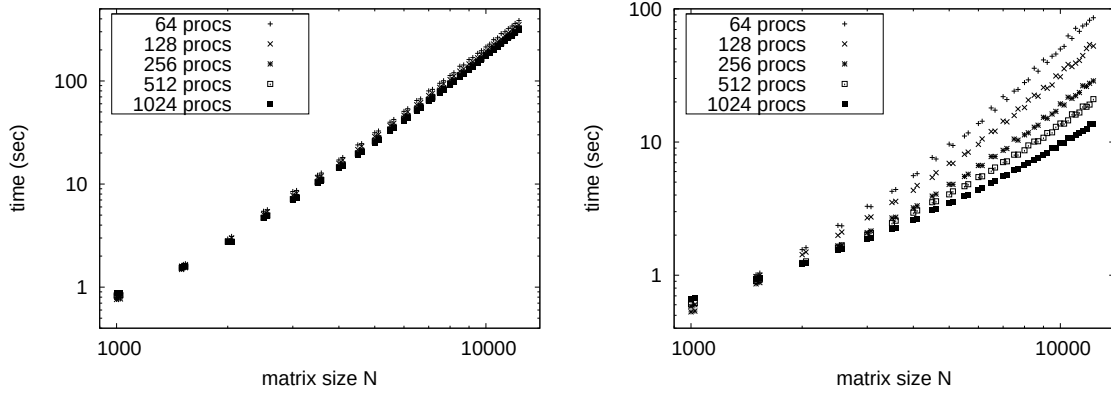
Figure 6: Run times computing ten percent of the eigenpairs of matrices with eigenvalues clustered around \varepsilon , using PDSYEVX (left) and PDSYEV (right).
