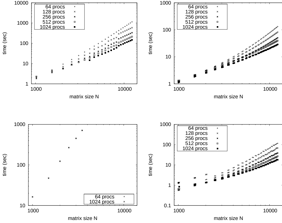
Figure 4: Run times computing all eigenpairs of matrices with eigenvalues clustered around \varepsilon , using PDSYEV (top left), PDSYEVD (top right), PDSYEVX (bottom left) and PDSYEVVR (bottom right).
