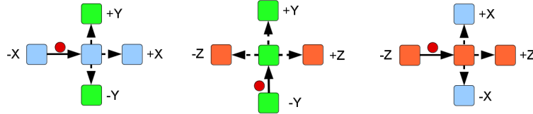
Figure 3: If a packet arrives at the receive link corresponding to -X direction it can be forwarded further along the X axis (being sent to the transmit FIFO corresponding to +X direction), or make a turn on in Y-direction.
