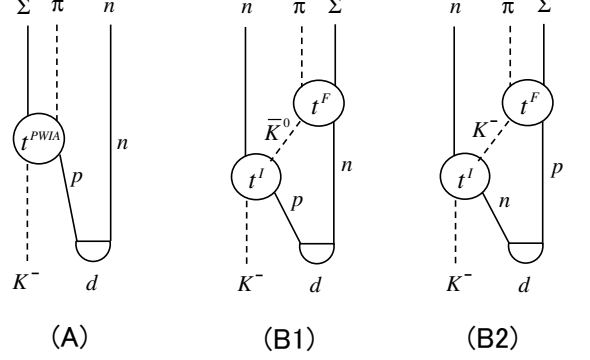
FIG. 3: Mechanisms included in our calculation of the reaction K^- d \rightarrow \pi\Sigma n . Plane-wave impulse-approximation (A); \bar{K}^0 n \rightarrow \pi\Sigma (B1) and K^- p \rightarrow \pi\Sigma (B2) rescattering, respectively.
