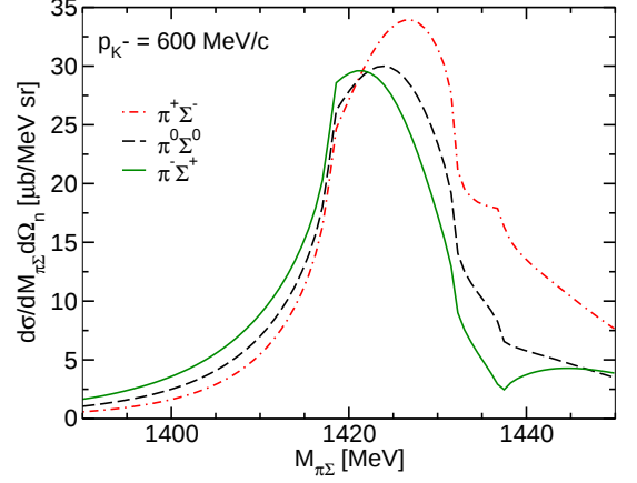
FIG. 11: \pi\Sigma invariant mass spectrum for the reaction K^-d \rightarrow \pi\Sigma n at the K^- beam momentum of 600 MeV/c and neutron angle \theta_n = 0^\circ . The results are based on the approximation Eq. (30) considering only the reaction mechanism B2. The K^-N \rightarrow \pi\Sigma amplitudes of the Oset-Ramos model [13] are used.
