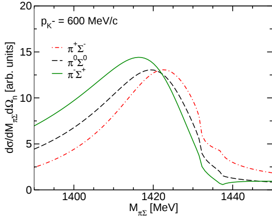
FIG. 10: \pi\Sigma invariant mass spectrum for the reaction K^-d \rightarrow \pi\Sigma n at the K^- beam momentum of 600 MeV/c and neutron angle \theta_n = 0^\circ . The results are based on using only t_{app}^F in Eq. (28) and considering only the reaction mechanism B2. The K^-N \rightarrow \pi\Sigma amplitudes of the Oset-Ramos model [13] is used.
