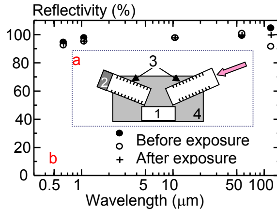
Fig.2. a) schematic of the new diagnostic duct for the retroreflector at LHD: 1) bending mirror, 2) flat mirror – a substitute of retroreflector, 3) diagnostic ducts with molybdenum fins and 4) the protecting housing. The direction of particle flux is shown with an arrow; b) dependence of the optical reflectivity on the wavelength for flat and bending mirrors before and after exposure in LHD.
