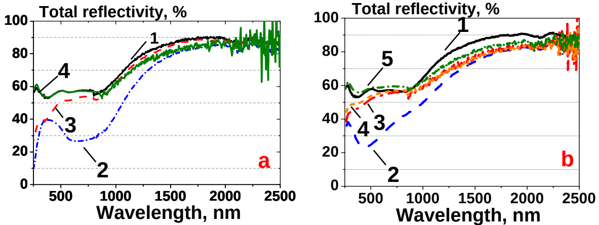
Fig. 3. Evolution of the total reflectivity after multiple cleaning treatments of mirrors contaminated in tokamaks: a) of the mirror with soft carbon film: 1) original clean mirror, 2) after deposition in the tokamak, 3) after 10 minutes of cleaning and 4) after 30 minutes of cleaning and b) of the Mo mirror with a hard carbon film: 1) original clean mirror, 2) after deposition in the tokamak, 3) after 35 minutes cleaning without biasing, 4) after additional biasing for 45 minutes and 5) after additional to 3) biasing for 256 minutes.
