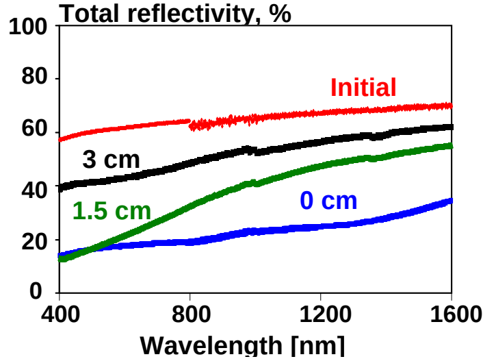
Figure 1. Reflectivity of mirrors from the divertor base located at the increasing distance from the plasma in channels. Shown is a distance from the entrance of the channel.
