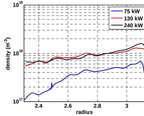
FIG. 1. radial electron density profiles measured by reflectometry in He-ICWC discharges in TORE SUPRA ( p=2 \cdot 10^{-2} Pa).
