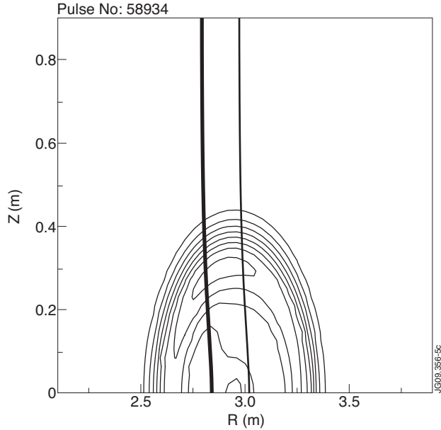
Figure 5: Showing the fast ion density across the R - Z plane according to Eqs. (21) for the latter part of Pulse No: 58934. The anisotropic distribution function recovers the local peaks in density, which are due to an abundance of trapped ions along lines tangent to the resonances. The location of the resonant field strengths are indicated with near vertical lines.
