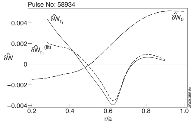
Figure 8: \delta \hat{W}_0 = \delta \hat{W}_{kt} + \delta \hat{W}_{fio} + \delta \hat{W}_{fp0} and \delta \hat{W}_{r1} according to Eq. (19), and also \delta \hat{W}_{r1} according to the fit of Eq. (29), plotted as a function of r_1 , for Pulse No: 58934.
