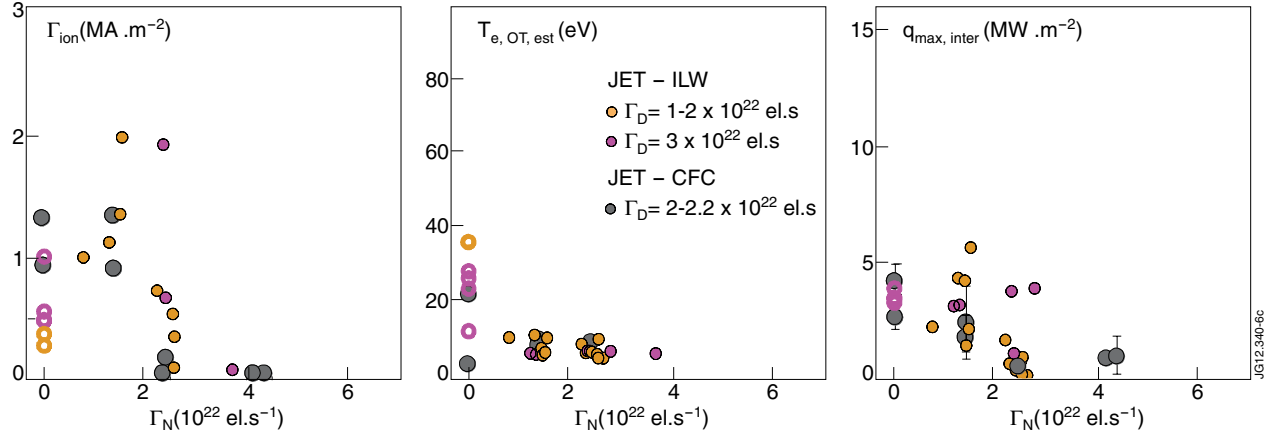
Figure 6: Ion current, electron temperature and peak power load at divertor outer target for JET-C and JET-ILW.
