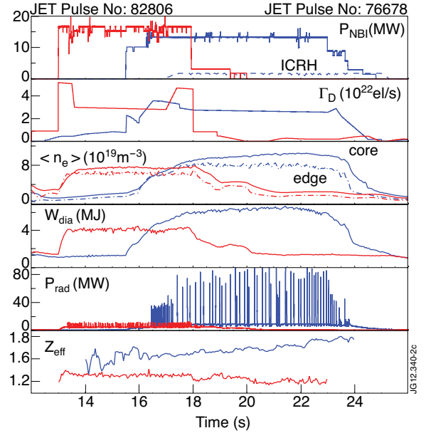
Figure 2: Time traces of unseeded ELMy H-mode discharges in JET-C wall Pulse No: 76678 (in blue), and JET-ILW Pulse No: 82806 (in red).
