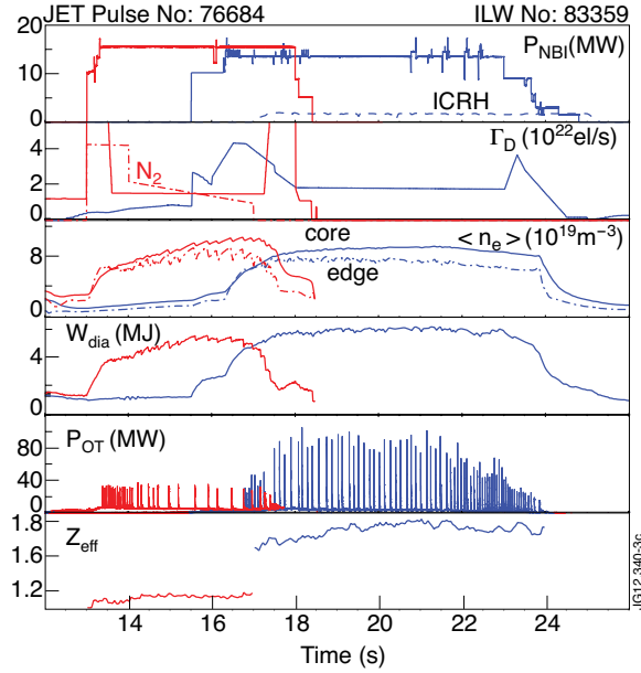
Figure 3: Time traces of unseeded ELMy H-mode discharges in JET-C wall Pulse No: 76684 (in blue), and N_2 -seeded JET-ILW Pulse No: 83359 (in red).
