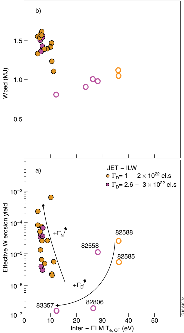
Figure 7: Effective W erosion yield a) and average pedestal stored energy versus target electron temperature in inter-ELM period b).
