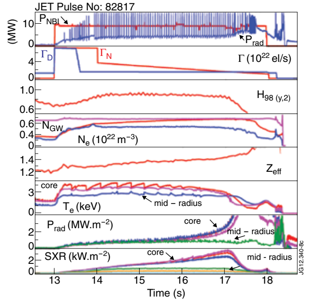
Figure 8: Time traces of N_2 -seeded ELMy H-mode discharges in JET-ILW wall Pulse No: 82817 (from top to bottom) NBI heating and total radiated power, D_2 and N_2 waveforms, normalized confinement factor H_{98} , core (red) edge (in blue) and Greenwald electron density (in pink), line-integrated Z_{eff} , electron temperature from core (in red and pink) and mid-radius (in blue), radiated power from core (in blue and pink) and mid-radius (in green) channel, and finally Soft x-ray radiated power.
