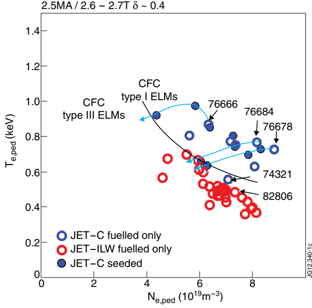
Figure 1: Pedestal n_e - T_e diagram for high ELMy H-mode discharges for JET-C and JET-ILW discharges with 2.5MA and 2-6-2.7T: JET-C discharges are in blue symbols, open if only fuelled and filled with the addition of N_2 seeding.
