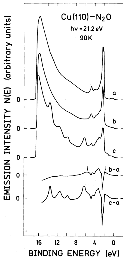
FIG. 1. He I UPS spectra [energy-distribution curves (EDCs)] with the sample at 90 K. a , clean Cu(110) surface; b , after a 0.4-L exposure to N 2 O; and c , after a 1-L N 2 O dosage. The difference curves are calculated with respect to the spectrum of the clean surface. In curve b — a the adsorbate-induced emission bands are indicated by arrows. The zero level of each spectrum is marked on the ordinate. All binding energies are referred to Fermi level.
