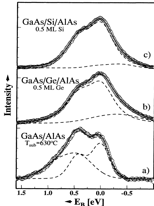
FIG. 3. Spectra of Ga 3d core levels ( h\nu = 48.37 eV) after background subtraction. The alignment corresponds to that of Fig. 1. Again, broken lines represent the different Ga 3d contributions whereas the solid lines represent the fitting results. (a) GaAs(100)/4 ML AlAs as in Fig. 1(c); (b) GaAs(100)/0.5 ML Ge/3 ML AlAs; (c) GaAs(100)/0.5 ML Si/3 ML AlAs. In all cases the AlAs overlayers were grown at T_{\text{sub}} = 630^\circ\text{C} .
