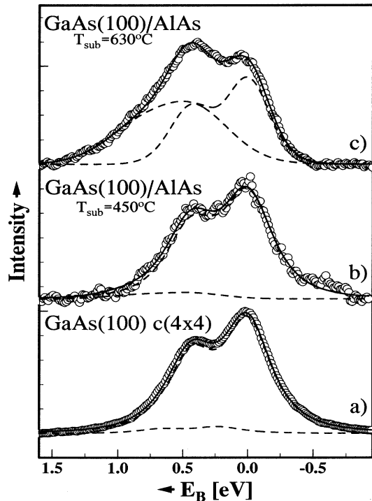
FIG. 1. Spectra of Ga 3d core levels ( h\nu = 48.37 eV) after background subtraction. In order to compensate for variations in band bending and work function the spectra were aligned along the Ga 3d bulk core level which was taken as the zero of the binding-energy scale. Broken lines represent the different Ga 3d contributions whereas the solid lines represent the fitting results. (a) GaAs(100) c(4 \times 4) substrate surface; (b) GaAs(100)/5 ML AlAs grown at T_{\text{sub}} = 450^\circ\text{C} ; (c) GaAs(100)/4 ML AlAs grown at T_{\text{sub}} = 630^\circ\text{C} .
