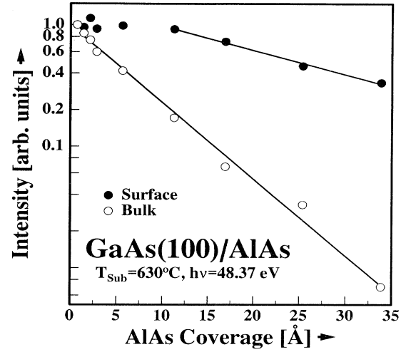
FIG. 2. Intensity of Ga 3 d surface and bulk components of GaAs(100)/AlAs heterostructures grown at T_{\text{sub}}=630^\circ\text{C} as a function of AlAs overlayer thickness.
