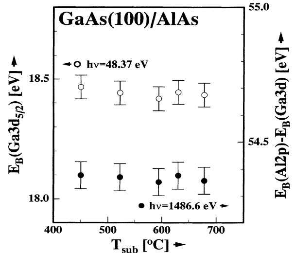
FIG. 4. Variation of Ga 3d to Al 2p and Ga 3d to VBM (AlAs) binding energy difference as measured with monochromatized XPS ( h\nu=1486.6 \text{ eV} ) and UPS ( h\nu=48.37 \text{ eV} ) on GaAs(100)/5 ML AlAs heterostructures for different AlAs growth temperatures. Any variation of the interface dipole or the band offset, \Delta E_v , should manifest themselves as variations in the values shown here.
