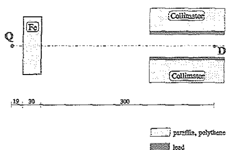
Fig. 1: Horizontal cross section of the benchmark geometry (Q: 14 MeV neutron source; D: detector; Fe: iron slab with dimensions of 100 \cdot 100 \cdot 30 \text{ cm}^3 )
