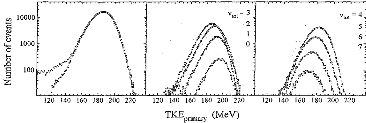
Fig. 3: Primary TKE spectra for ^{252}\text{Cf} (see text).
