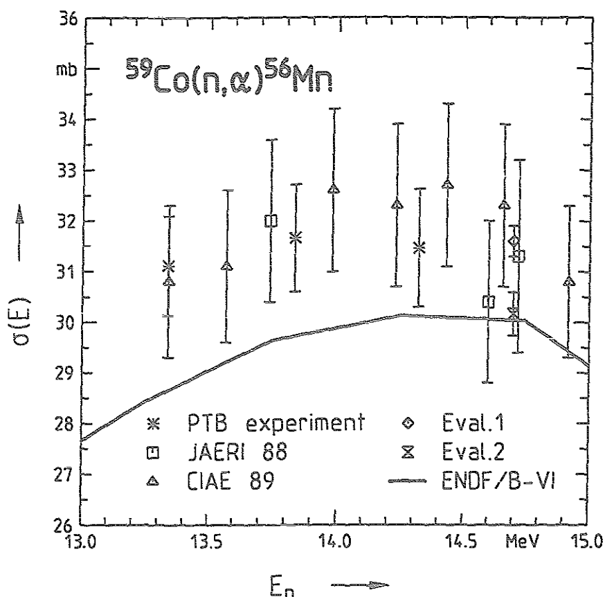
Fig. 3 Cross section of the ^{59}\text{Co}(n,\alpha)^{56}\text{Mn} reaction around 14 MeV.
