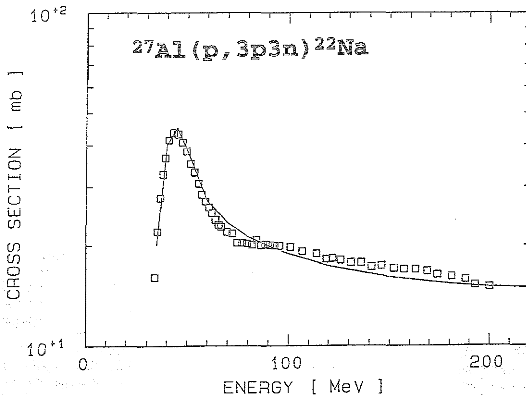
Fig. 1: Excitation function for the production of ^{22}\text{Na} from proton irradiation of aluminum as recommended by Tobaillem et al. [8] (full line) and as measured recently by Steyn et al. [9] (open squares).
