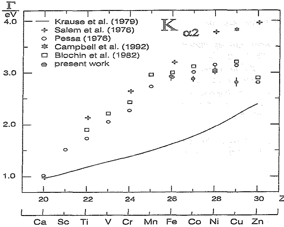
Figure 2: K_{\alpha 2} widths of X-ray lines in the region of 3d elements.
