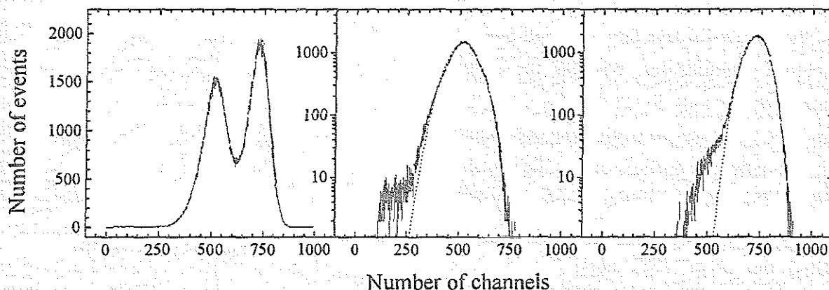
Fig. 1: Kinetic energy spectra for ^{252}\text{Cf} (see text).
