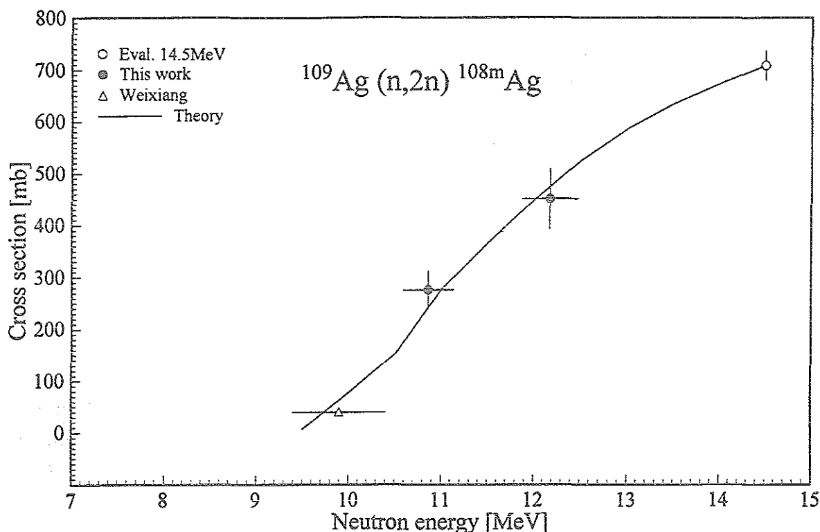
Fig. 2 Excitation function of the ^{109}\text{Ag}(n,2n)^{108\text{m}}\text{Ag} process.
