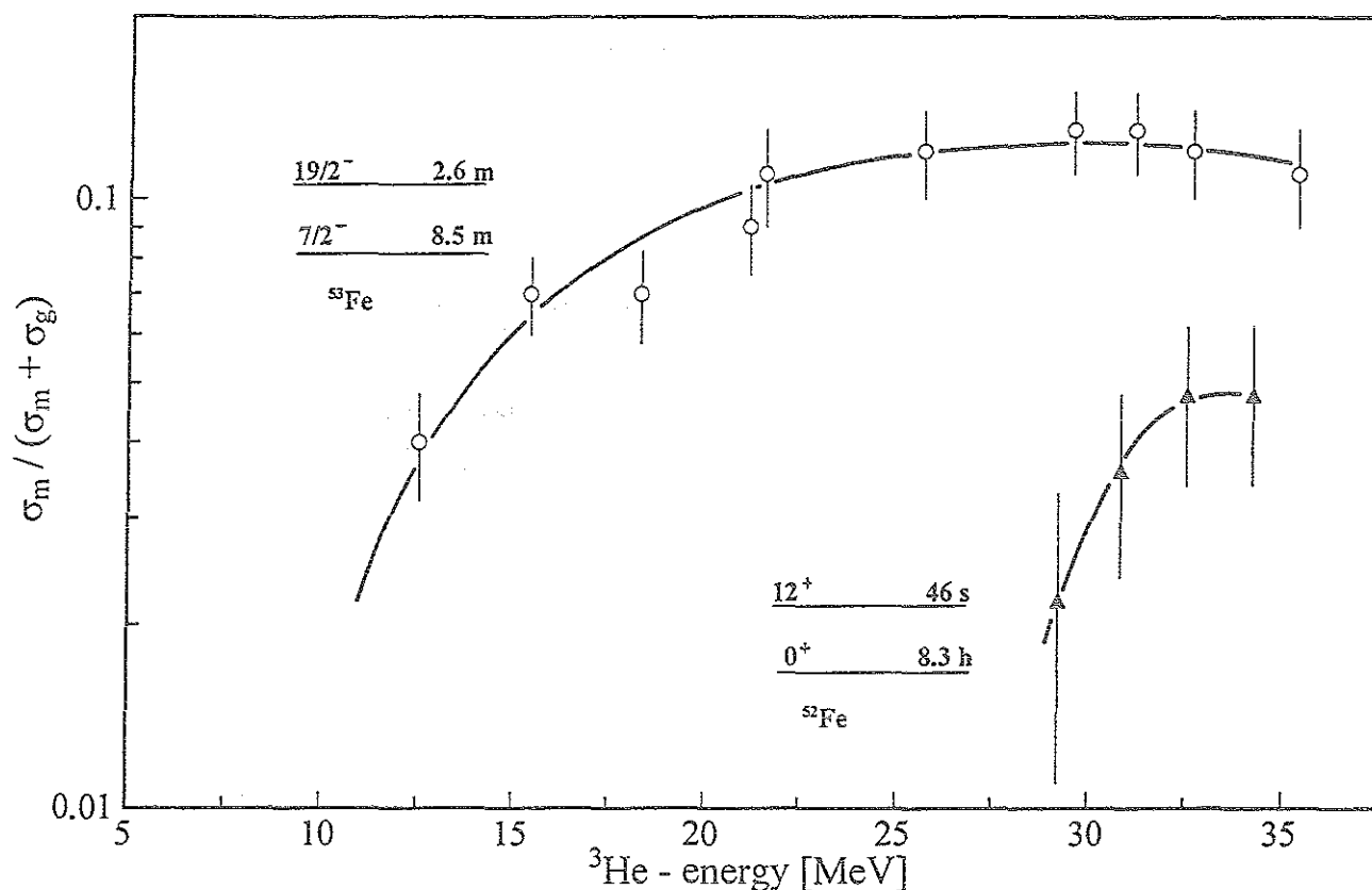
Fig. 1 Isomeric cross section ratios for the isomeric pairs ^{52m,g}\text{Fe} and ^{53m,g}\text{Fe} produced in (^3\text{He}, \text{xn}) reactions on ^{52}\text{Cr} .
