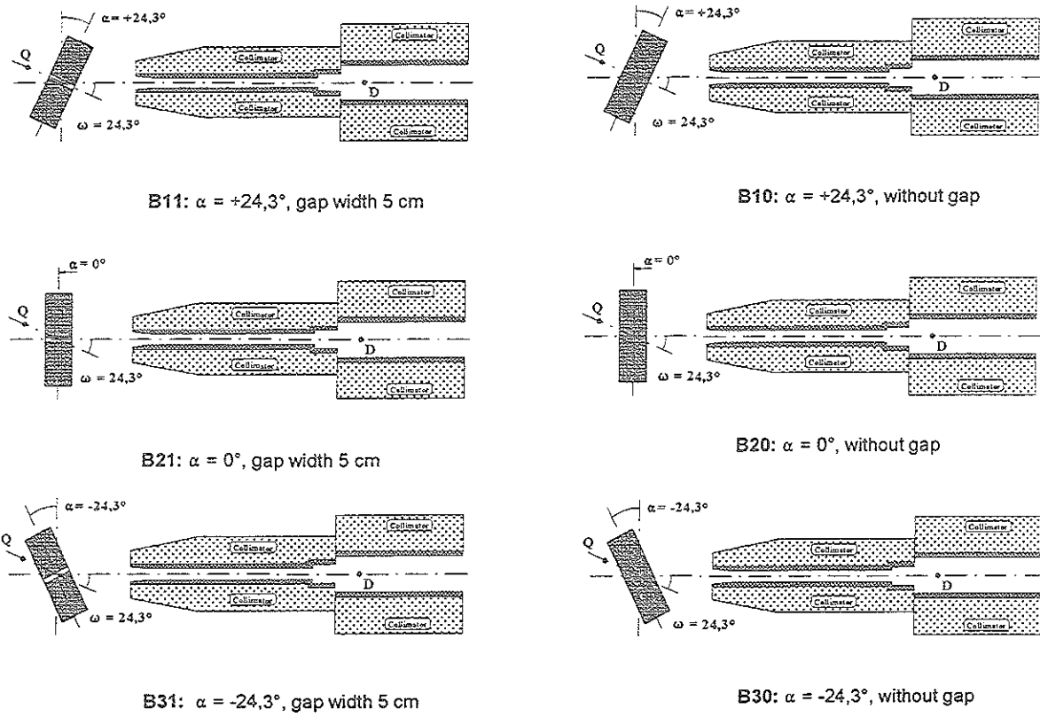
Fig. 1: Geometries investigated ( Q: 14 MeV neutron source, D: detector )
