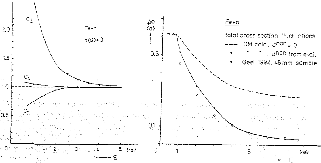
Fig. 1 (left) - First three correction factors in Eq. 1 for an iron sample, effective thickness three mean paths ( n\langle\sigma\rangle = 3 ), with moments obtained from Geel data in \pm 10\% energy windows.
