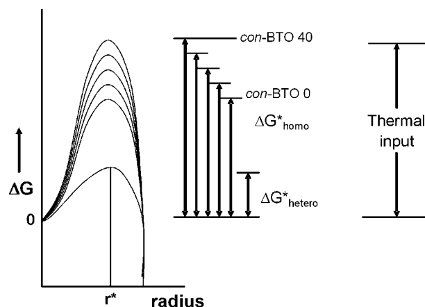
Fig. 8 Schematic for the hypothetical change of free energy barriers for homogeneous ( \Delta G^*_{\text{homo}} ) and heterogeneous ( \Delta G^*_{\text{hetero}} ) nucleation depending on the amount of con -BTO addition to the \mu E-BTO dispersion. r^* represents the critical radii for nuclei growth. As indicated in the text the barrier height for \Delta G^*_{\text{hetero}} is kept constant to simplify the diagram. Besides the different barrier heights on the right hand side the amount of available thermal energy input is plotted. In the case of con -BTO 40 the latter is barely sufficient to surmount the energy difference for the homogeneous nucleation. Thus depending on the kinetics a columnar (Fig. 2d, RTA process) and a polycrystalline (diffusion furnace), respectively, morphology is obtained.
