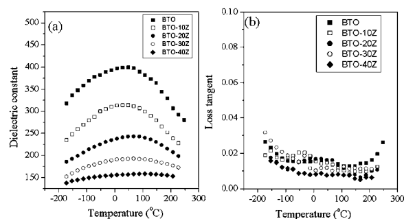
Fig. 6 Temperature dependent (a) dielectric constant and (b) loss tangent of BTO films with various ZrO_2 contents measured at 10 kHz.
