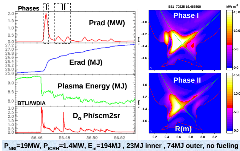
Fig.2 Typical large ELM radiation distribution
