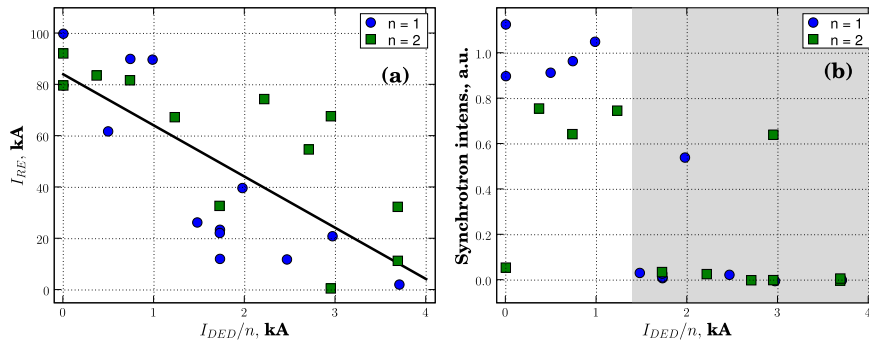
Figure 4: Suppression of runaway electrons by resonant magnetic perturbations. a - dependence of the runaway current on the RMP amplitude. b - dependence of the synchrotron emission ( \lambda = 3 \div 5 \mu\text{m} ) on the RMP amplitude.
