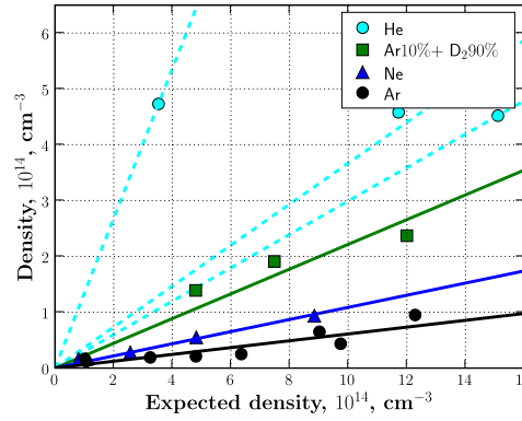
Figure 3: Mixing efficiency for different gases.
