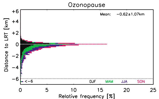
Figure 12. Relative frequency histogram of MOZAIC ozonopauses [Bethan et al. , 1996] related to the LRT for different seasons based on the time period 2001–2008.
