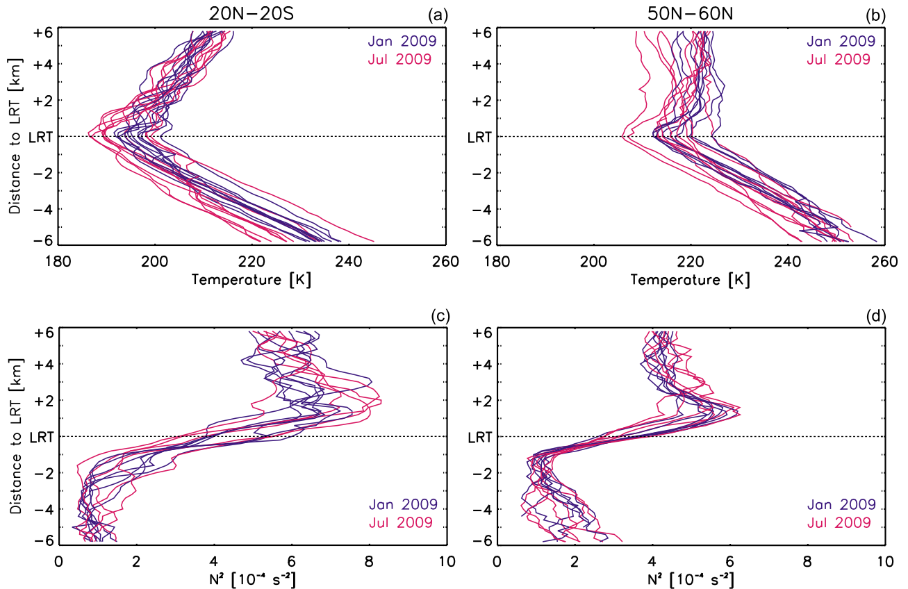
Figure 6. Examples of (a, b) individual temperature and (c, d) N^2 profiles from GRACE for the tropics (Figures 6a and 6c) and midlatitudes (Figures 6b and 6d) for January (blue) and July (red) 2009. The vertical coordinate is tropopause-based.
