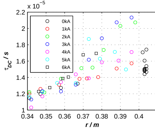
Figure 3: Turbulence decorrelation is increasing towards the plasma edge. For low 2 \leq I_{DED} < 3 kA a increase of 25% is measured at the plasma edge.
