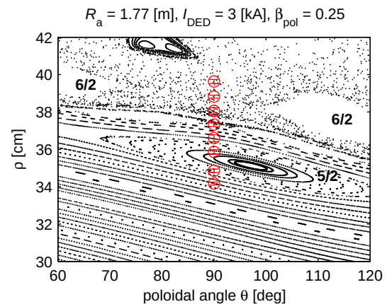
Figure 1: Detail of a Poincare Plot with observation radii of reflectometry. The diagnostic covers the 6/2 and 5/2 island chains
