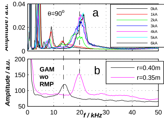
Figure 6: Amplitude spectrum of Mirnov coil (a) and reflectometry (b) showing the correlation between both diagnostics for a case without RMP and with RMP.
