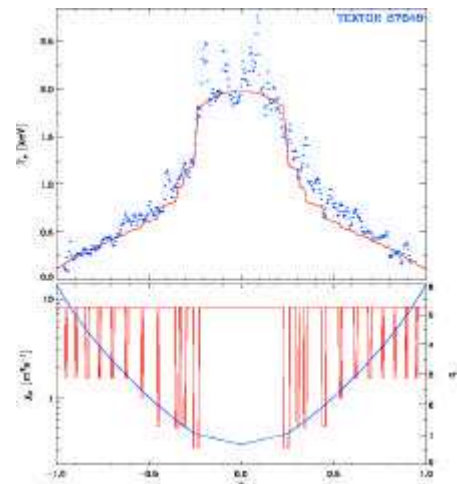
Fig.1 The T_e profile in a typical TEXTOR discharge with central 250 kW ECRH simulated with the RTP q -comb model for the electron heat conductivity. Blue dots represent measured T_e . The red curve gives the result of the simulation. The bottom panel shows the q profile (blue) and the corresponding profile of the electron heat conductivity \chi_e .
