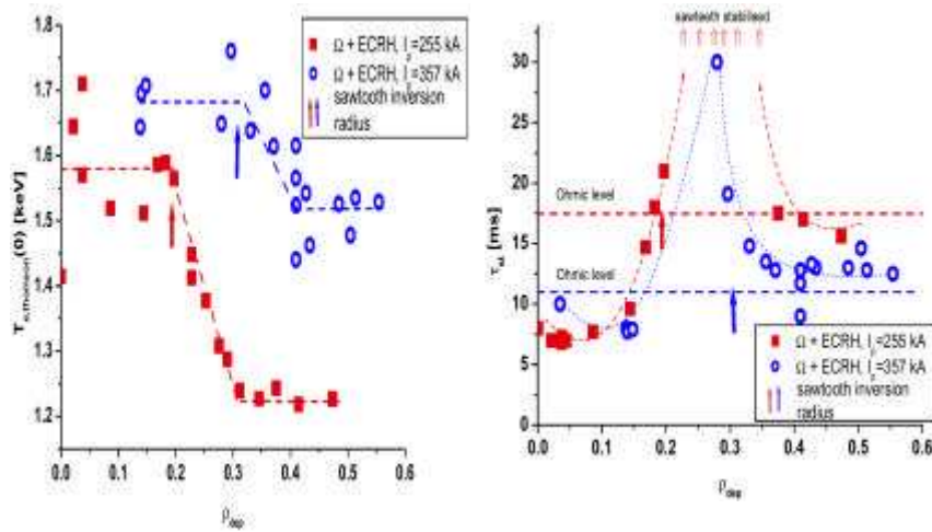
Fig. 2 The central T_e and the corresponding sawtooth period achieved in Ohmic discharges with ECRH as a function of the ECRH deposition radius. The ECRH deposition radius is varied by changing the toroidal field. Two datasets are shown: squares for I_p=255 kA and circles for 357 kA. In the lower current case sawteeth are stabilised, when ECRH is deposited within a region just outside the sawtooth inversion radius.
