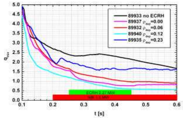
Fig. 6 The evolution of the minimal safety factor for discharges with different location of the ECR heating. The time at which q_0=1 drops below 1 is qualitatively consistent with appearance of sawteeth.
