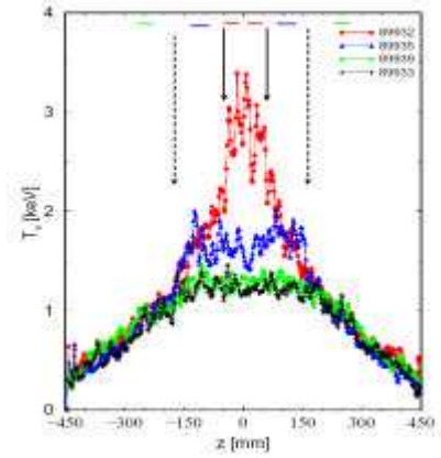
Fig. 4: T_e profiles from Thomson scattering at t=0.35 s for different positions of ECRH deposition: 89932 \rho_{\text{dep}}=0.06 ; 89935 \rho_{\text{dep}}=0.23 ; 89939 \rho_{\text{dep}}=0.50 ; 89933 NBI-only.
