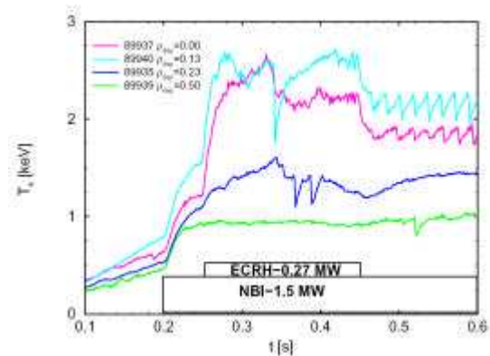
Fig. 7: Time traces of the electron temperature for various ECR heated discharges, with different deposition: 89937: \rho_{\text{dep}}=0.0 , 89940 \rho_{\text{dep}}=0.13 , 89935: \rho_{\text{dep}}=0.23 and 89939: \rho_{\text{dep}}=0.50 . Note the large crash for 89940 and the appearance of sawteeth for rather centrally heated discharges and the absence of them for off-axis heating. The crashes in 89935 are most probably caused by MHD activity at q=1.5 .
