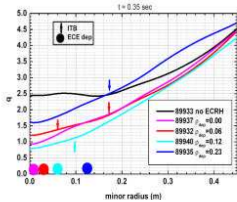
Fig. 5: q profiles as calculated with the ASTRA code at the time of Thomson Scattering. Observed barriers are indicated by arrows and are close to rational q -values: q=1, 1.5, 2, 2.5 . Note that central shear is not negative..
