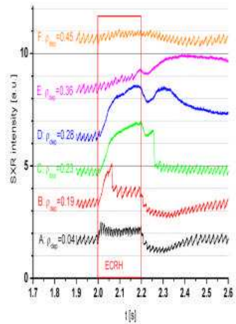
Fig. 3: Time traces of the SXR intensity for discharges differing in EC deposition radius. For central deposition (A) the sawtooth period is shortened. For heating outside the inversion radius (C-E) sawteeth are stabilised. The discharges remain in the non-sawtooth regime even after switch off of ECRH. For D and E the SXR intensity is about a factor of 2 higher than in the ohmic case before ECRH. Note the crashes in B and C after which the discharges return to the normal sawtooth regime.
