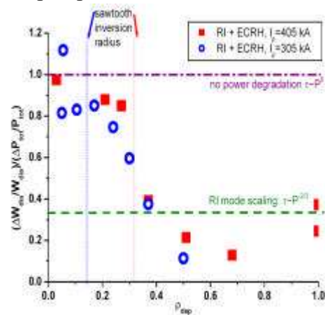
Fig. 8: Normalised efficacy of ECRH in RI-mode discharges for two different currents. A transport barrier close to the inversion radius might be recognized. For heating inside this transport barrier no power degradation is observed.
