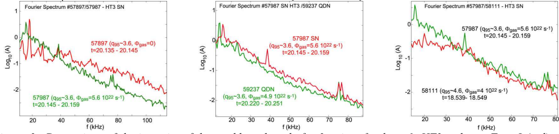
Figure 3: Comparison of the intensity of the washboard mode for 3 pairs of pulses: 1. HT3 at low q Type I (red) and Type II (green), 2. SN vs. QDN at 2.5MA/2.7T, Type II phases, and last to the right, HT3 at low and high q_{95} . The low q pulse in plot 3 has mixed Type I-II ELMs. Note that the high frequency part of the spectrum is similar for both q_{95} , but the high q_{95} lacks the enhanced MHD at low frequency, typical of Type II ELM phases.
