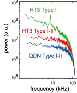
Figure 7: intensity of the density fluctuations for pulses 57897 (green), 57987 (red), and for comparison, the QDN 2.5MA/2.7T, 59237 (blue)
