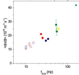
Figure 9: particle refuelling rate vs. Type I ELM frequency, for the same set of data as figure 8.
