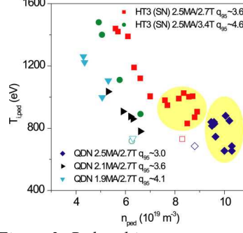
Figure 2: Pedestal ion temperature vs density for the same plasmas of fig. 1.
