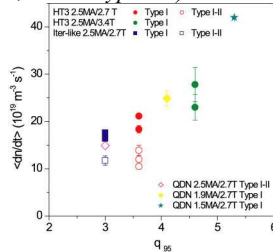
Figure 8: comparison of the particle re-fuelling rate between Type I ELMs for various plasma conditions.
