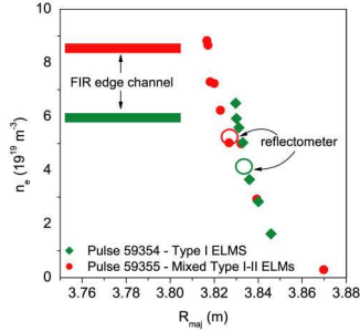
Figure 6: position of the cut-off density gradient region for 59354/57897 (SN, Type I) and 59355/57987 (SN, mixed Type I-II).
