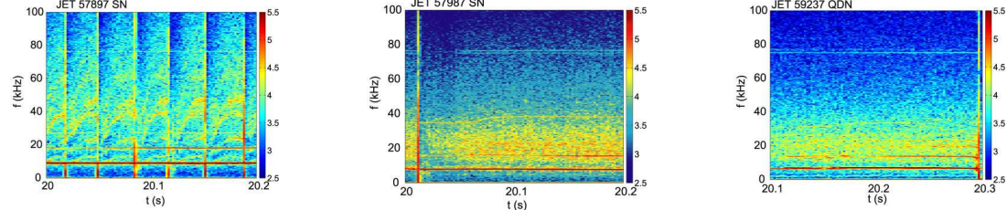
Figure 4: Spectrogrammes for 3 of the plasma discharges described above: SN HT3 2.5MA/2.7T Type I; in the middle HT3 2.5MA/2.7T with Type II ELMs, and last QDN at 2.5MA/2.7T with Type II ELMs. The intense and narrow vertical bands are type I ELMs, the horizontal continuous modes are correlated to sawtooth activity.
