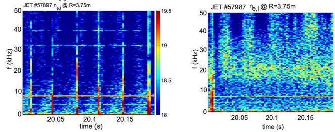
Figure 5: density fluctuation measurement in SN, type I (left), and mixed Type I-II (right). Same discharges as for figure 4, plots 1 and 2.
