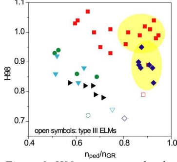
Figure 1: H_{98} vs n_{ped} normalised to n_{GR} . Same legend as fig 2.
