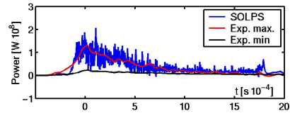
Figure 8. Evolution of the power onto the outer divertor during the ELM.
