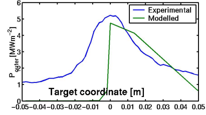
Figure 5. Outer divertor heat flux profile in stationary conditions from model and Infra Red themography
