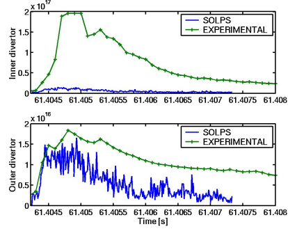
Figure 6. D_\alpha signal at the inner and outer divertor. The code fails to reproduce the target asymmetry
