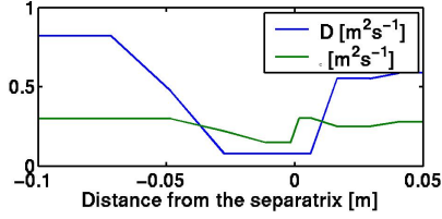
Figure 1. Particle ( D ) and energy ( \chi ) diffusivity profiles
