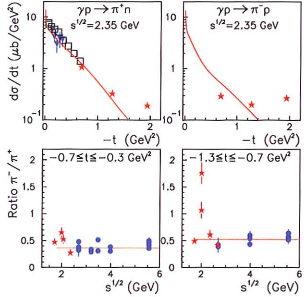
Fig. 30: Differential cross sections for charged pion photoproduction for center-of-mass energy 2.35 GeV as a function of the momentum transfer squared (upper panels) and the ratio of \pi^- to \pi^+ production (lower panels) as a function of the center-of mass energy. The squares and crosses show the world data obtained before 1980. The recent Hall A data are given by stars. The solid line represents the new Regge approach.
