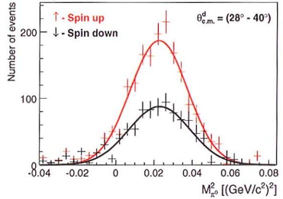
Fig. 14: Angular dependence of the missing-mass squared distribution for the reaction d\bar{p} \rightarrow dp_{sp}X measured with the storage cell and 1.2 GeV deuteron beam. Red and black histograms stands, respectively, for data with target polarization 'spin-up' and 'spin-down', after background subtraction using N_2 data.
