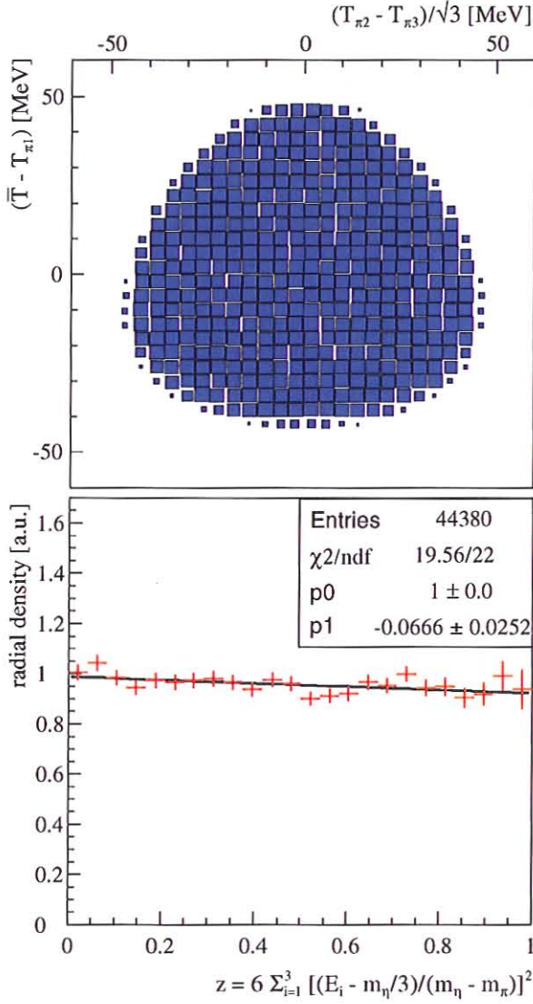
Fig. 17: Efficiency corrected symmetrized Dalitz plot of the \eta \rightarrow 3\pi^0 decay from WASA-at-COSY data (top) and radial density distribution for the extraction of the slope parameter \alpha (bottom).
