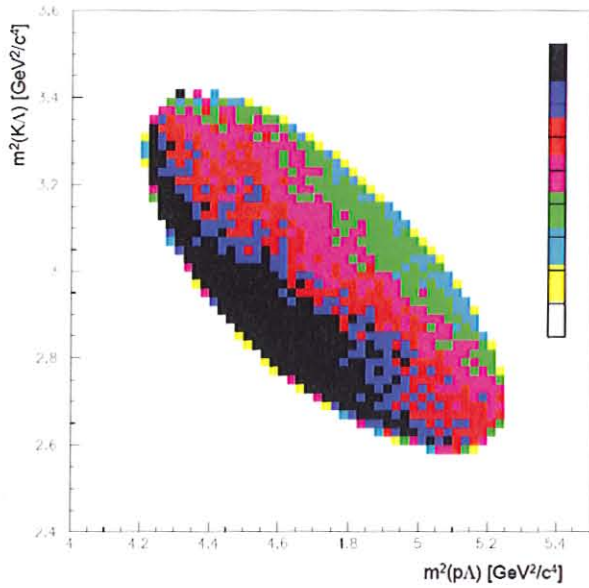
Fig. 15: Preliminary Dalitz plot of the reaction pp \rightarrow pK^+\Lambda for a beam momentum of 3.06 GeV/c. The sample contains about 320,000 events covering the full phase space.
