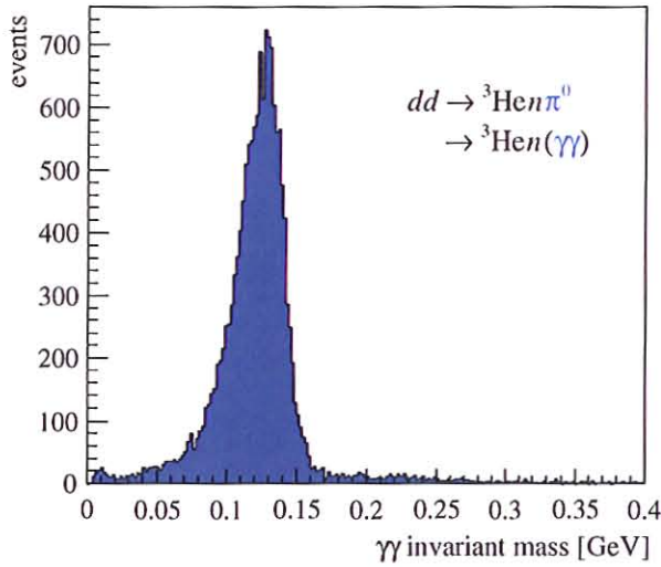
Fig. 19: \gamma\gamma invariant mass for events with ^3\text{He} nuclei identified from the energy loss information in the WASA Forward Detector from approximately seven hours of data taking at T_d = 351 MeV, corresponding to the reaction dd \rightarrow ^3\text{He} n \pi^0 .
