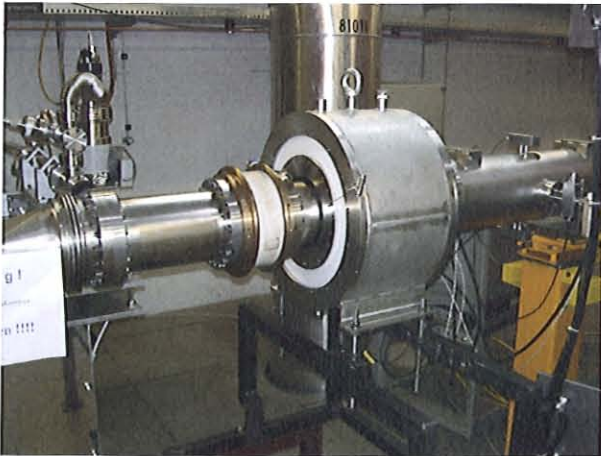
Fig. 50: The barrier bucket cavity with its asymmetric layout is installed in one arc of COSY. In this figure the shielding of the gap is dismantled to make it visible.
