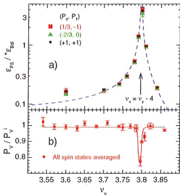
Fig. 36: (a) Ratio of \epsilon_{FS} to *\epsilon_{Bdl} is plotted vs. the vertical betatron tune \nu_y ; \Delta f was 300 Hz; the cooling was off. (b) Measured deuteron vector polarization ratio at 1.85 GeV/c is plotted vs. \nu_y ; the rf dipole was off, the cooling was on. The red curve is a fit to a 2 nd order Lorentzian.
