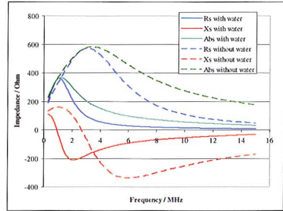
Fig. 43: Measurements of the cavity impedance with and without water cooling showing the resistive (Rs) and the reactance (Xs) components as well as the magnitude of the impedance (Abs).
