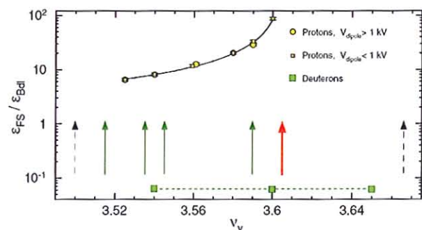
Fig. 35: Ratio of \epsilon_{FS} to \epsilon_{Bdl} is plotted vs. vertical betatron tune \nu_y . The betatron beam resonances are shown by the black dashed arrows; the 1 st and 3 rd order proton spin resonances are shown by the red and green arrows, respectively.
