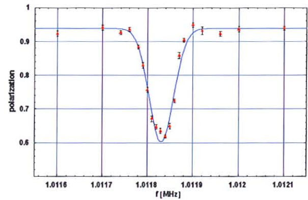
Fig. 39: Example of a measured resonance curve. The plot shows the measured vector polarization versus frequency of the rf-solenoid.
