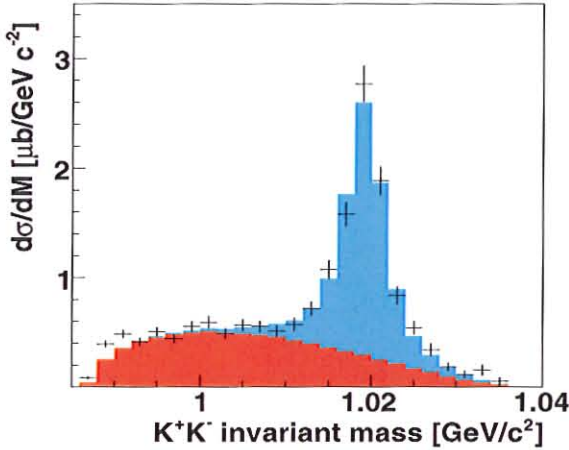
Fig. 3: Differential cross section for the pp \rightarrow ppK^+K^- reaction at 2.65 GeV as a function of the K^+K^- invariant mass compared to Monte Carlo simulations of \phi (blue) and non- \phi (red) contributions.
