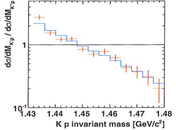
Fig. 4: Ratio of the differential cross sections for the pp \rightarrow ppK^+K^- reaction at 2.65 GeV away from the \phi region as function of the K^-p and K^+p invariant masses. Experimental data (red) are compared to a Monte Carlo simulation (blue).
