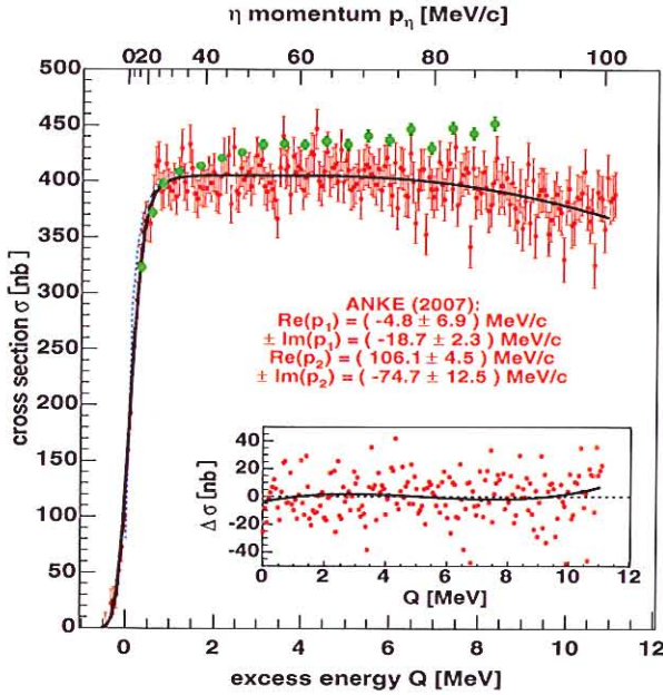
Fig. 1: ANKE (red) and COSY-11 measurements of the dp \rightarrow {}^3\text{He}\eta total cross section in terms of the excess energy Q and c.m. \eta momentum p_\eta . The line corresponds to the two-pole fit of Eq. (1). The inset shows the deviation of the ANKE data from the fitted line.
