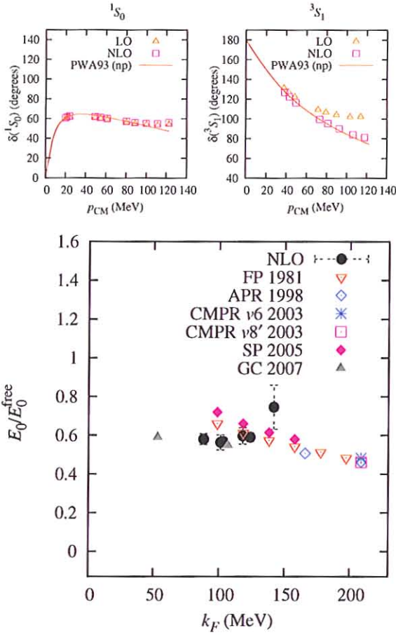
Fig. 29: Upper panel: S-wave phase shifts versus center-of-mass momentum for LO 2 (triangles) and NLO 2 (squares) compared to the Nijmegen partial wave analysis (solid lines). Lower panel: Results for the ground state energy E_0 at NLO (normalized to the free energy E_0^{\text{free}} ) versus the Fermi momentum k_F (black circles with error bars). For comparison, we show results available in the literature based on different methods.
