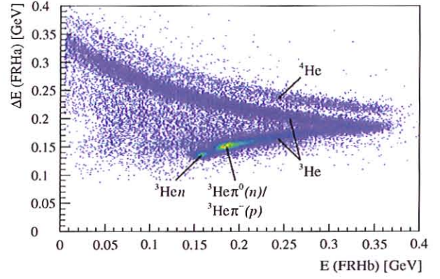
Fig. 18: \Delta E -E plot from the first two FRH layers FRHa and FRHb at T_d = 1117\text{ MeV} . Bands for {}^3\text{He} and {}^4\text{He} are clearly separated. Structures for fast {}^3\text{He} correspond to the binary dd \rightarrow {}^3\text{He}n breakup channel and quasi-free single pion production.
