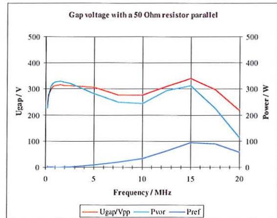
Fig. 44: First high power tests at the barrier bucket cavity showing the nearly frequency independent peak to peak gap voltage (red) together with the forward power (light blue) and the reflected power (dark blue).
