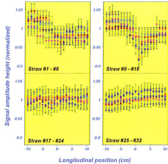
Fig. 55: Measured efficiency along the tube for all 32 straws. The beam hit all tubes around 0 cm.
