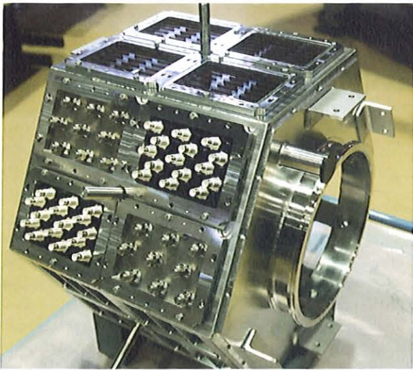
Fig. 16: The hexagonal vacuum vessel, which allows for the lead through of more than 3000 signal lines, high-voltage cables, and gas tubes.
