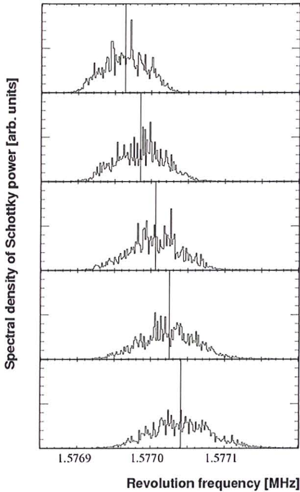
Fig. 41: Frequency distributions of the Schottky noise power measured during one ten-minutes cycle. The frequency shift is positive because these data were taken above the transition energy of the accelerator. Each spectrum is generated within 2 s. The time difference between consecutive spectra shown here is two minutes. The time dependence of the shift of the mean frequency over the cycle is a measure for the target thickness.
