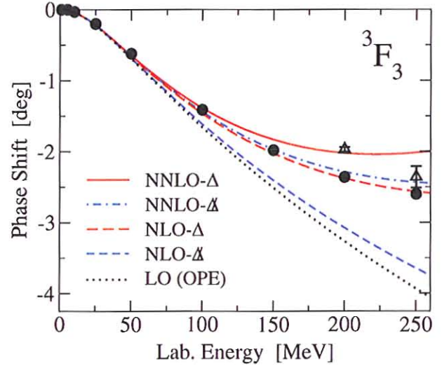
Fig. 28: {}^3F_3 NN phase shift in EFT with and without explicit \Delta 's calculated in first Born approximation using the spectral-function cutoff 700 MeV. The filled circles (open triangles) depict the results from the Nijmegen (Virginia Tech) PWA.
