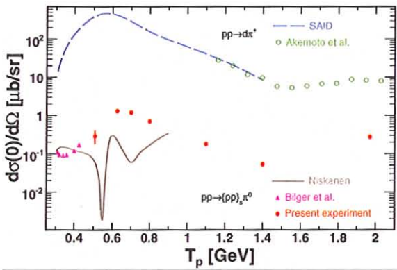
Fig. 7: Energy dependence of the differential cross section for the pp \rightarrow \{pp\}_s\pi^0 reaction with E_{pp} < 3 MeV. The closed circles represent the ANKE results while the triangles show the low energy CELSIUS data. The solid curve corresponds to the prediction from the model of J.A. Niskanen. For comparison the cross section for the pp \rightarrow d\pi^+ reaction is shown: the dashed curve is the SAID parameterization, the open circles depict the KEK results.
