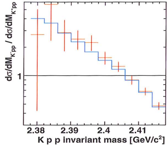
Fig. 5: Ratio of the differential cross sections for the pp \rightarrow ppK^+K^- reaction at 2.65 GeV away from the \phi region as function of the K^-pp and K^+pp invariant masses. Experimental data (red) are compared to a Monte Carlo simulation (blue).
