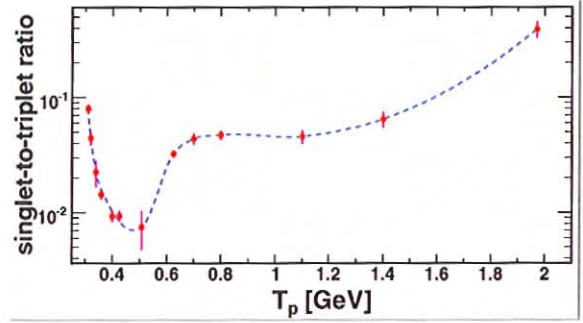
Fig. 8: Ratio of the single-pion production cross sections associated with formation of spin-singlet and spin-triplet nucleon pairs. The curve is to guide the eye.
