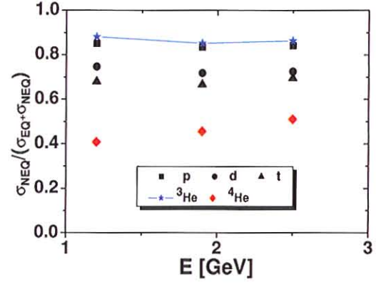
Fig. 10: Ratio of non-equilibrium processes (coalescence & "fireball") to total cross sections (non-equilibrium & evaporation) as function of beam energy.
