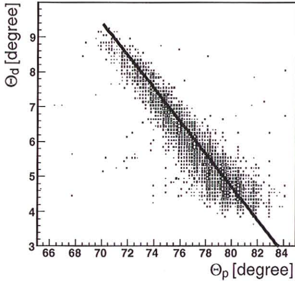
Fig. 12: Angular correlation between the protons and deuterons detected in the STT and forward detector, respectively. The expected kinematical correlation for the dp elastic reaction is shown by the black line.
