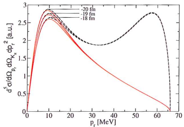
Fig. 27: Sensitivity of the differential cross section for the reaction \gamma d \rightarrow \pi^+ nn to the nn scattering length a_{nn} . The solid and dashed lines correspond to the angular configurations with \theta_r = 90^\circ and \theta_r = 0^\circ , respectively. The different values of a_{nn} used are specified in the figure.
