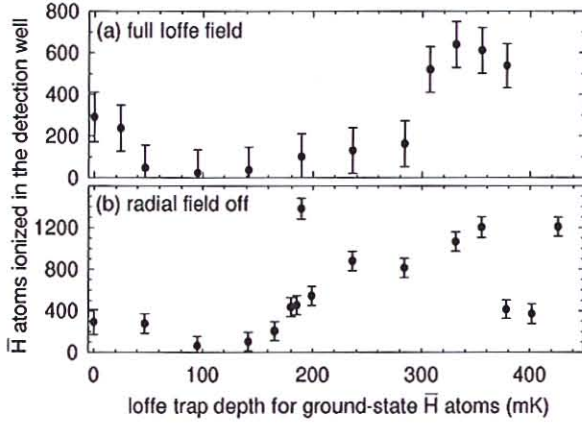
Fig. 26: Detected \bar{H} atoms vs. its depth, for (a) a complete Ioffe trap and (b) only pinch coils being energized.
