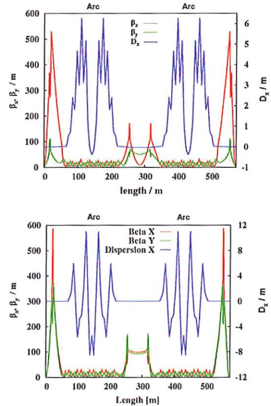
Fig. 42: Optical functions for the HESR superconducting 4 fold symmetry (bottom) and normal conducting (top) magnet lattice from Table 1. Shown are the horizontal betatron amplitude \beta_x (red), the vertical betatron amplitude \beta_y (green), and the horizontal dispersion D_x (blue) along the ring.
