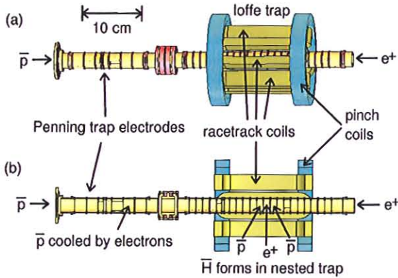
Fig. 24: Outside (a) and cross section (b) view of the ring electrodes from the Penning trap, overlaid by the quadrupole Ioffe trap.
