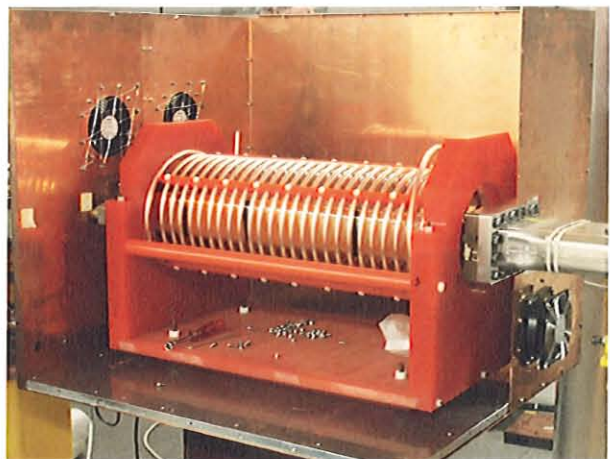
Fig. 37: The water-cooled rf solenoid; its longitudinal rf magnetic field integral is 1.95 T mm peak-to-peak.
