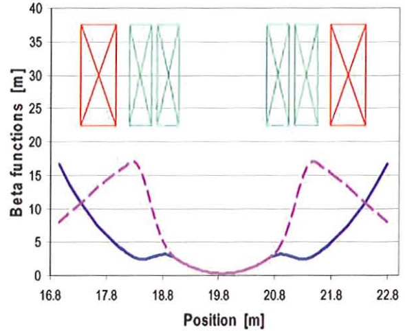
Fig. 20: The geometry of the low- \beta (large acceptance) section around the target at COSY. The storage cell (see below) will be located in the center between the four additionally needed magnets. The lines denote the vertical (dashed line) and horizontal (solid line) beta function, proportional to the size of the beam.
