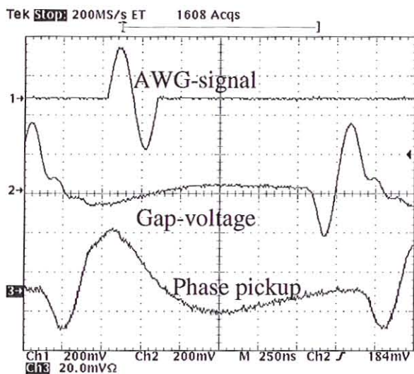
Fig. 46: Single sinusoidal starting signal, corresponding gap voltage and beam distribution measured with a phase pickup.
