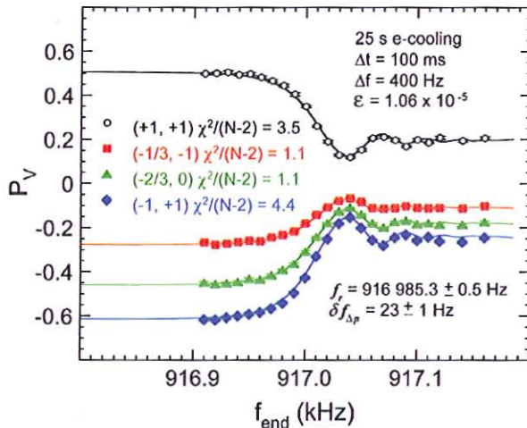
Fig. 38: Vertical vector polarization ( P_V ) of 1.85 GeV/c stored deuterons plotted vs the end-frequency of the 400 Hz sweep; this and other fits give precise measured values of: resonance strength ( \pm 0.5\% ), frequency spread ( \pm 1 Hz), and f_r ( \pm 0.00005\% ).
