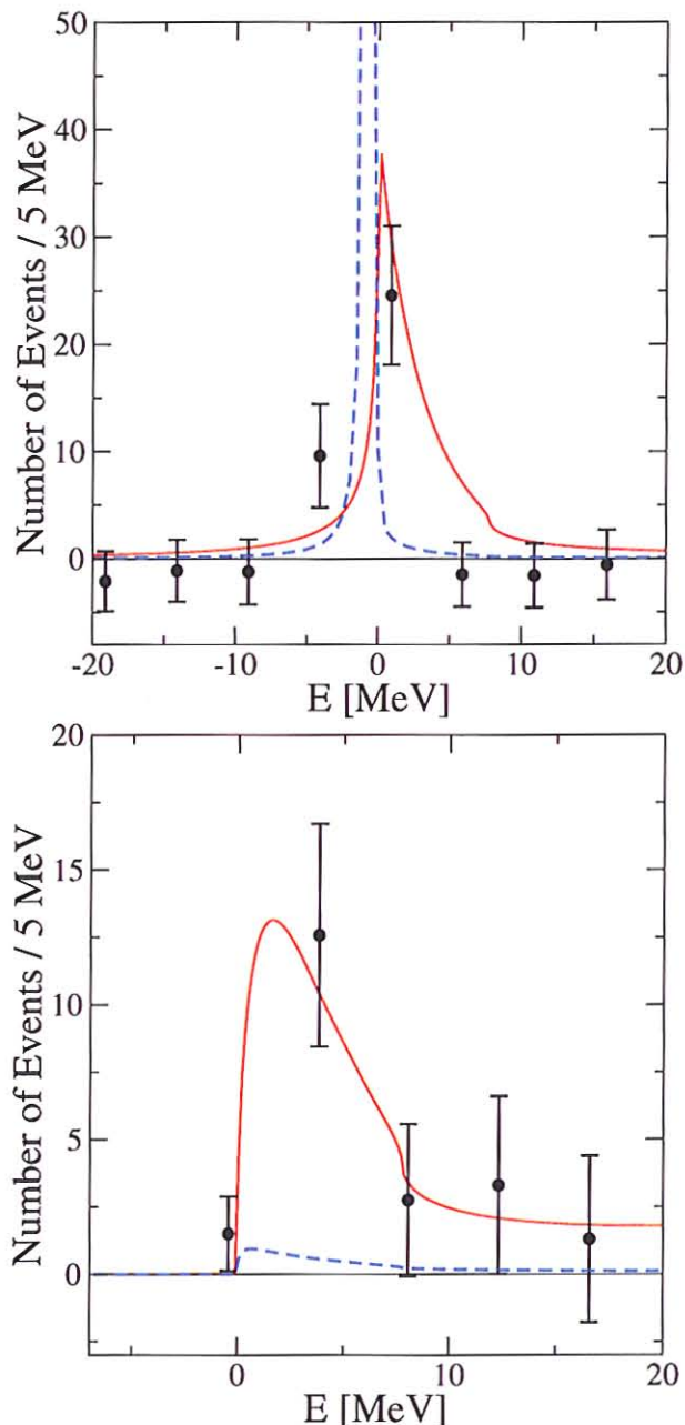
Fig. 31: Upper panel: comparison of our best fit (solid, red curve) to the data in the J/\psi\pi^+\pi^- channel. The data are from Belle. The dashed, blue line is the result, when the pole is moved on the physical sheet. integrated over the given bins. Lower panel: Belle data in the \bar{D}D\pi channel. Lines as above.
