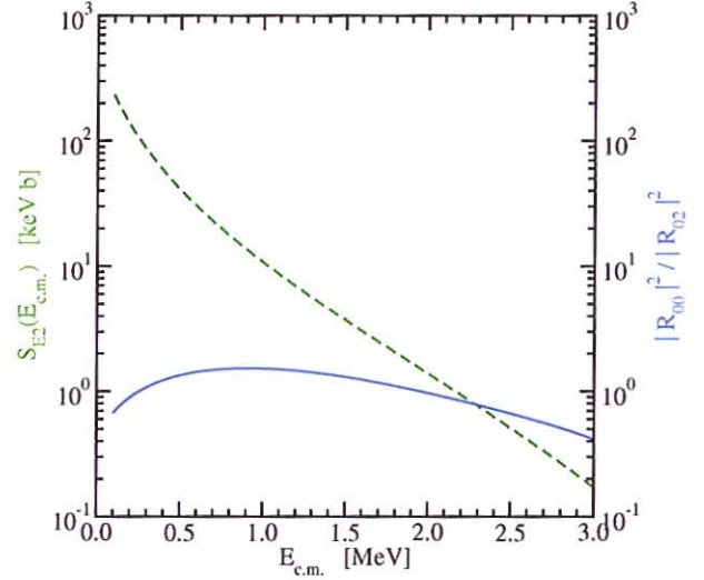
Fig. 32: Dashed curve and left scale: E2 S-factor; solid curve and right scale: E0/E2 radial matrix element ratio, vs. E_{\text{c.m.}} .
