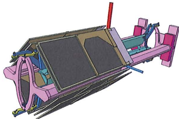
Fig. 23: The openable storage cell with the surrounding silicon detectors.
