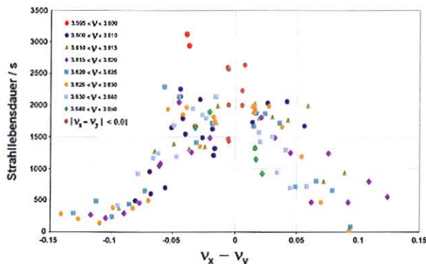
Fig. 40: Measured beam lifetime in seconds versus tune.
