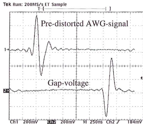
Fig. 47: Pre-distorted barrier bucket signal and the corresponding gap-voltage.
