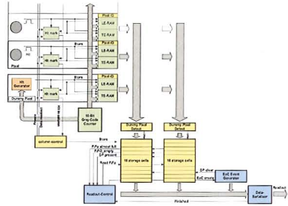
Fig. 51: Readout scheme for the front-end electronics of the pixel part of the MVD.
