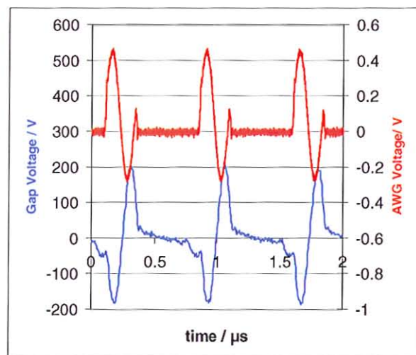
Fig. 48: Solid state amplifier input signal (dc plus single sinus) and corresponding gap-voltage.
