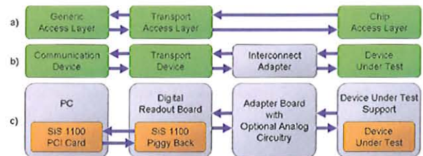
Fig. 52: Readout chain. a) shows the abstract model of the software modules, b) the abstract model of the hardware devices and c) shows the actual setup.
