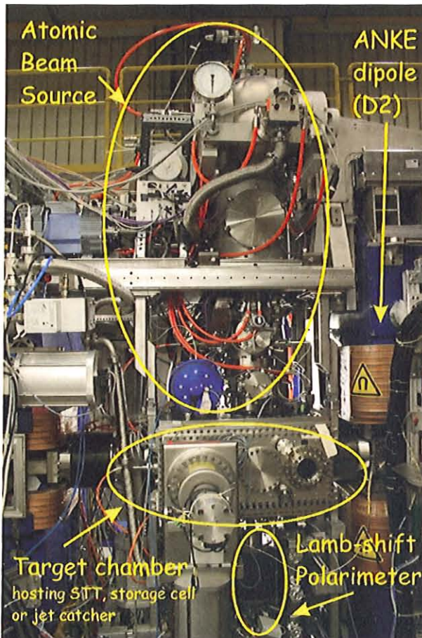
Fig. 11: Photo of ANKE with the Polarized Internal Target (PIT) in front of the spectrometer dipole D2. The main components of the PIT system: Atomic Beam Source (ABS), Lamb-shift Polarimeter (LSP), and the target chamber hosting Storage Cell (SC) together with Silicon Tracking Telescope (STT) system are indicated.
