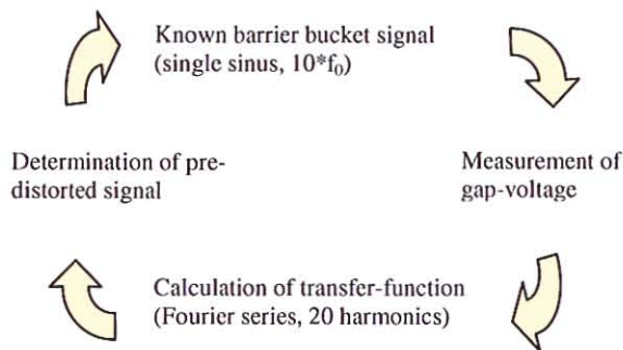
Fig. 45: Schematics of signal synthesis.
