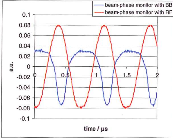
Fig. 49: Barrier bucket bunch (blue) in comparison with a bunch in a single harmonic cavity (red).
