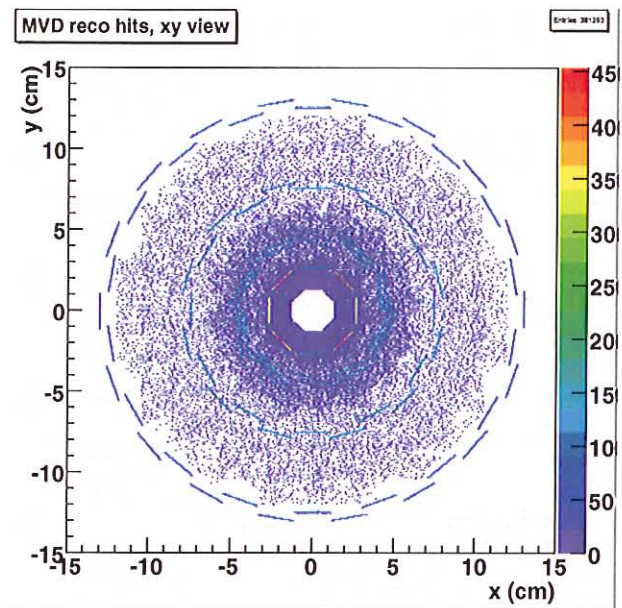
Fig. 53: Position of the reconstructed points projected onto the xy-plane
