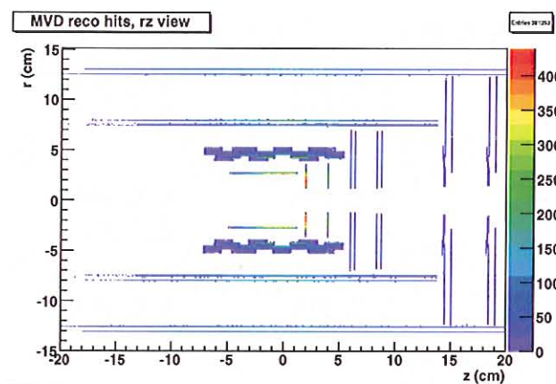
Fig. 54: Position of the reconstructed points projected onto the rz-plane
