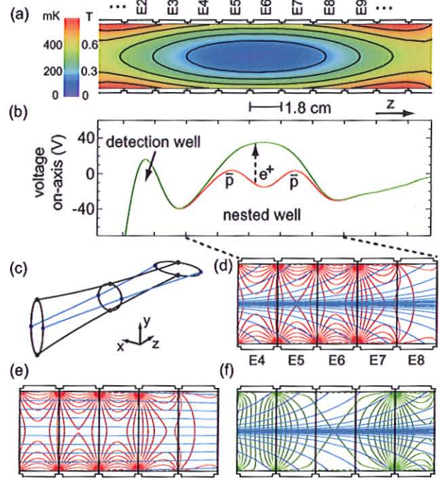
Fig. 25: Well depth and field distributions in the electrodes.
