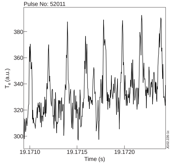
FIG. 2. ECE channel at R = 3.84 m.
