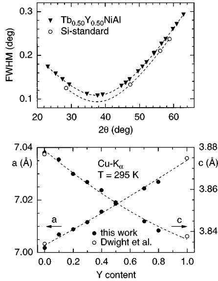
FIG. 2. Overview of the x-ray data obtained for the series \text{Tb}_{1-x}\text{Y}_x\text{NiAl} . The measured linewidth (FWHM) is shown for a representative compound and the NBS Si standard (upper panel). The composition-dependent lattice constants (measured at room temperature) are given in the lower panel. Note that a increases with increasing Y content x whereas c decreases. The data from Dwight et al. 3 for TbNiAl and YNiAl are included. The dashed lines are guides to the eye.
