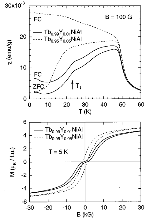
FIG. 3. The dc susceptibility of \text{Tb}_{0.99}\text{Y}_{0.01}\text{NiAl} and \text{Tb}_{0.95}\text{Y}_{0.05}\text{NiAl} measured at increasing temperature in a constant magnetic field of B = 100 G (with both FC and ZFC history) is shown in the upper panel. At the temperature T_1 a change in the antiferromagnetic order of \text{Tb}_{0.99}\text{Y}_{0.01}\text{NiAl} occurs. In the lower panel the magnetization curves of the same compounds at a constant temperature of T = 5 K are given.
