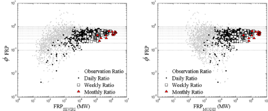
Figure 5.14: Ratios of FRP, \phi_{FRP} , as a function of the FRP measured by SEVIRI (left) and MODIS (right). Ratios are identical to those presented in Figure 3, and are separated by the width of the temporal window in which the fire pixels were aggregated; either on an observational ( n=2239 ), daily ( n=365 ), weekly ( n=52 ), or monthly basis ( n=12 ).
