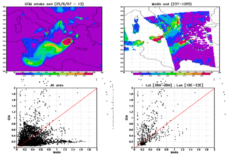
Figure 5.48: Modelled smoke AOD [-] (left) and observed MODIS AOD [-] product (right) for Aqua overpasses on 25 August, 1205UTC (top). AOD scatter plots for the entire area and a box on the fire Greek plume (bottom).
