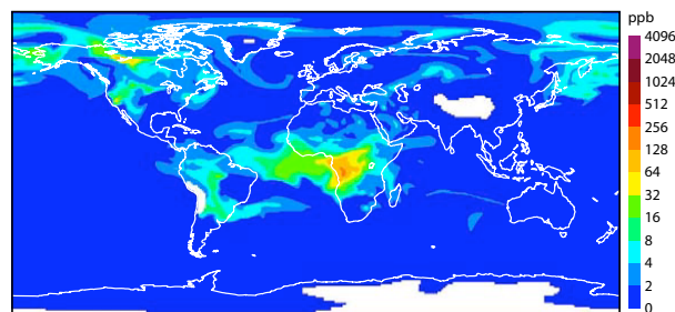
FIGURE 2. 48-hour atmospheric fire plume forecast, valid on 30 July 2008, 0000 UTC: CO [ppb] on 700 hPa pressure level.
