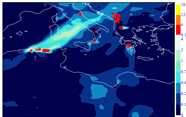
Figure 5.51: Modelled organic matter plus black carbon AOD [-] (bluish) on 30 August 2007, 1430UTC, overlaid with observed SEVIRI FRP [W/m2] interpolated to model resolution (reddish). The University of Lecce AERONET station is indicated by a white circle.
