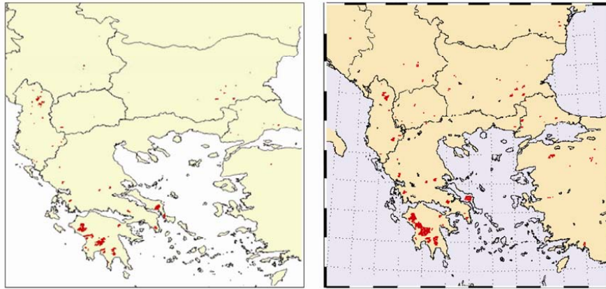
Figure 5.46: Active fires (hotspots) detected by MODIS (left) and by SEVIRI (right) on August 25, 2007 over the Mediterranean region.
