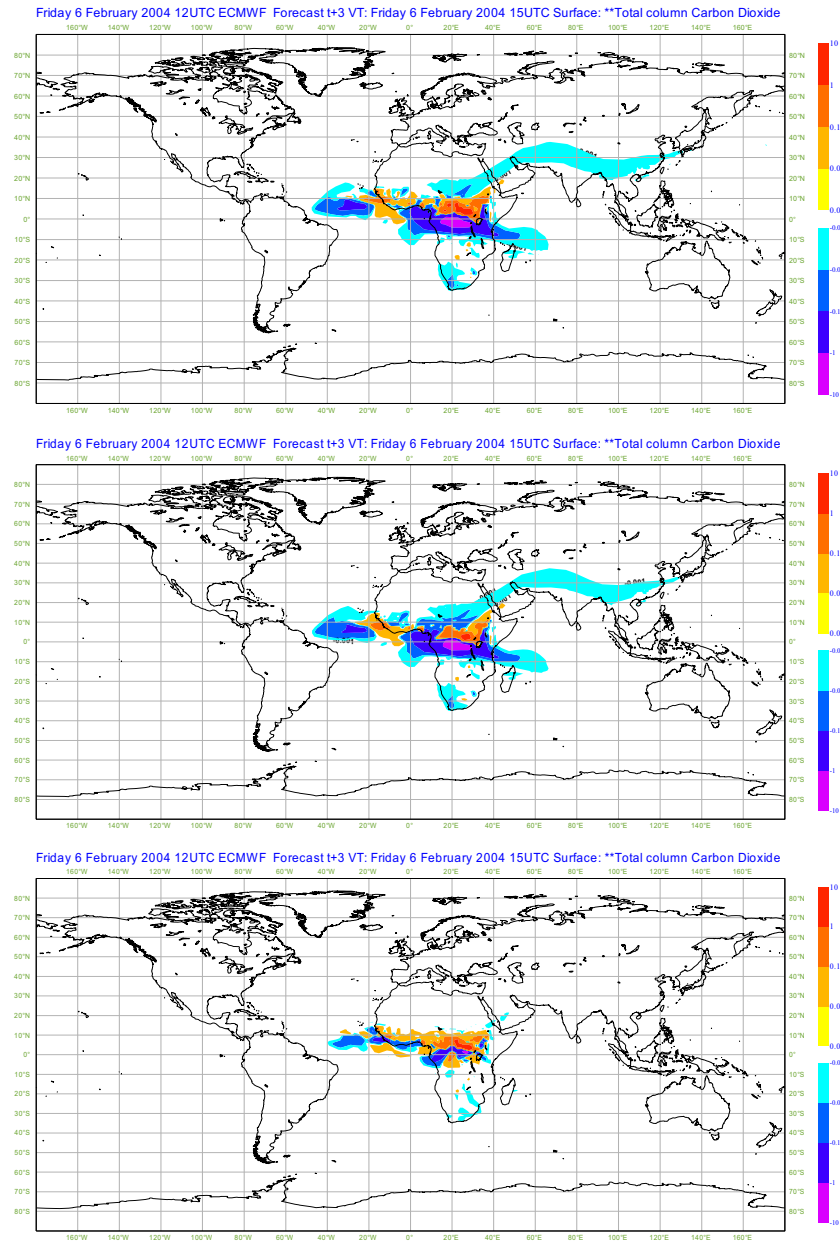
Figure 5.38: Differences in fire contribution to total column CO 2 for emissions with different time resolutions: 1h - 8d (top, Figure 5.37 top - bottom), 1d - 8d (middle), 1h - 1d (bottom).
