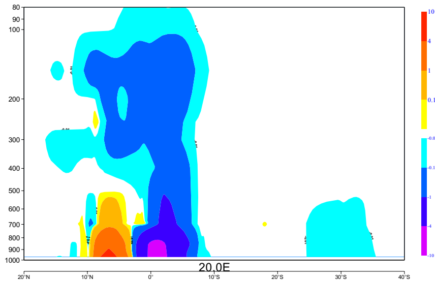
Figure 5.39: Vertical distribution of difference in fire contribution to the CO 2 mixing ratio for emissions with different time resolutions of 1-hour and 8-days.
