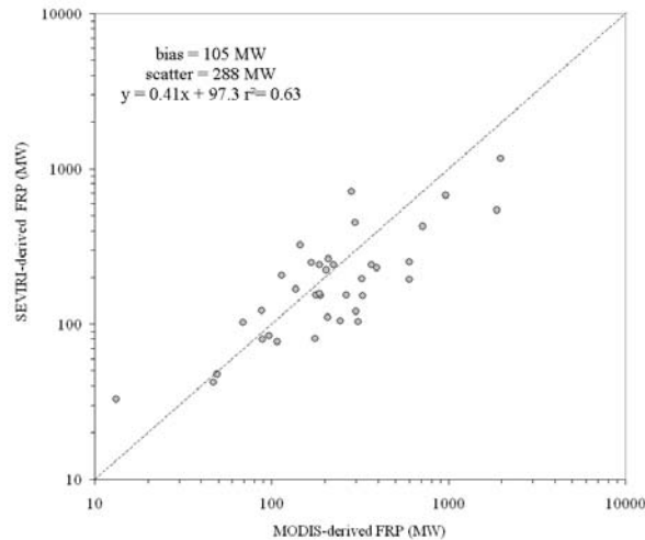
Figure 5.34: A comparison of per-fire FRP derived from SEVIRI and MODIS observations of fires observed near-simultaneously by each sensor over South America. Fires are designated as contiguous clusters of active fire pixels and SEVIRI FRP measured were taken from the Land SAF FRP per-pixel products of South America collected in July 2007.
