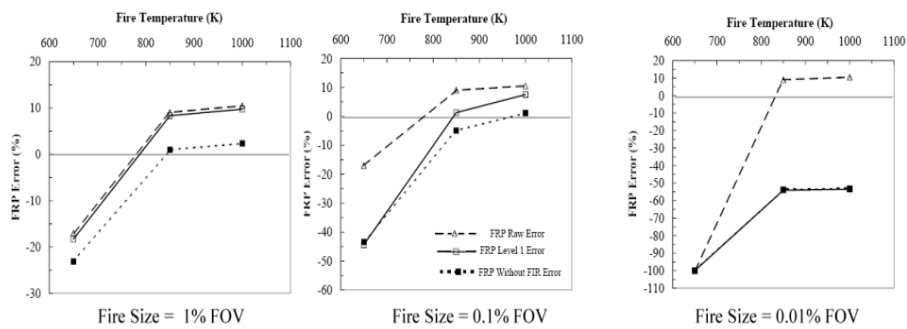
Figure 5.27: The effect of the SEVIRI observation process on the retrieval of FRP for fires of different effective temperatures and pixel proportions. The errors in FRP is shown due to the fourth order approximation to the Planck function only, to the complete modelled level 1 observations process (PSF and FIR filter) and to the observations without the FIR filter.
