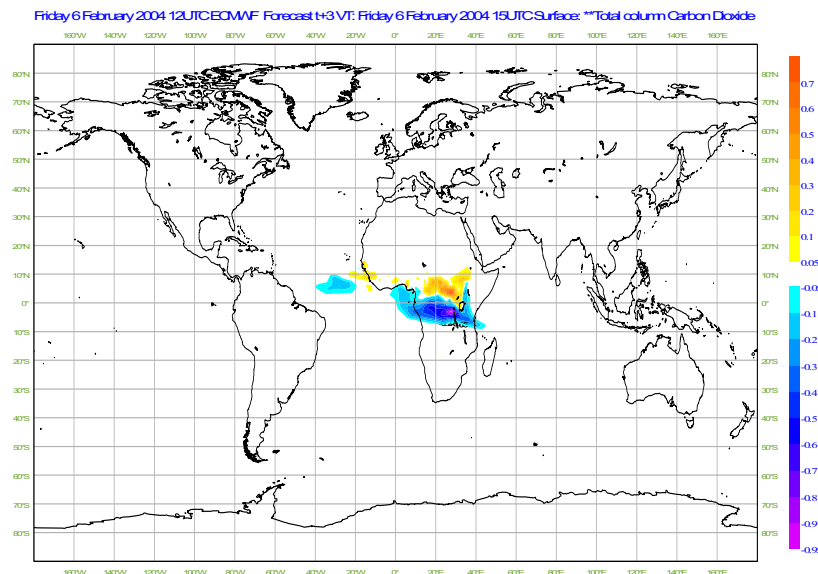
Figure 5.40: Relative difference of total column \text{CO}_2 for different time resolutions. (1\text{-hourly} - 8\text{-daily fires [ppm]}) / (1\text{-hourly} - \text{no fires} + 1 \text{ ppm}) .
