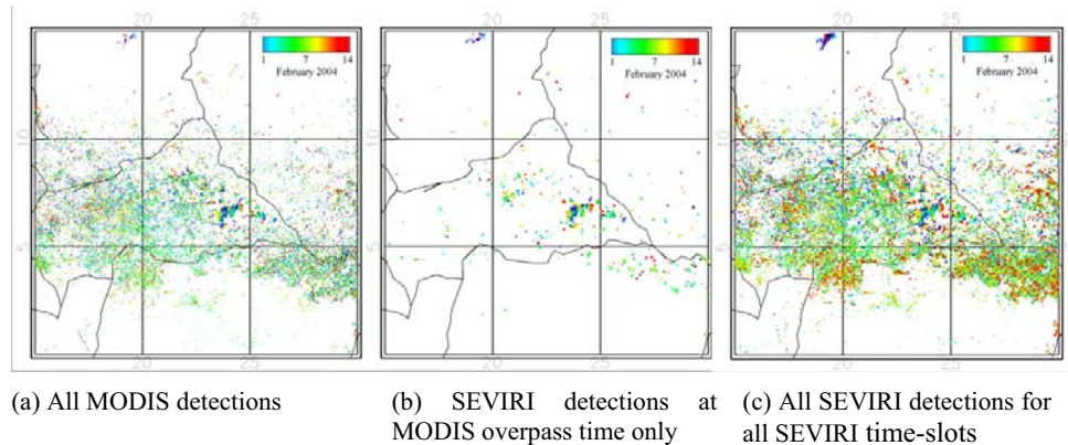
Figure 5.8: Effect of the inability of SEVIRI to detect low FRP fire pixels that MODIS can detect, illustrated by SEVIRI and MODIS fire detections collected over Central African Republic and surroundings in February 1-14 2004. Fire pixel detections are coloured by day of detection. When only using data from the SEVIRI imaging slots that were co-incident with a MODIS overpass, comparison of (b) with (a) confirms that SEVIRI misses a large number of (low FRP) fire pixels. However, it should also be noted that when using all SEVIRI imaging slots, SEVIRI appears to agree well in comparison to MODIS in terms of identifying the spatial distribution fire-affected areas, and in fact can detect a larger number of fires overall. The conclusion is that whilst many fires have an insufficiently high FRP to be detected by SEVIRI if we limit the SEVIRI observations to just those at the MODIS overpass time, most fires appear to become sufficiently large and intense at some point in their lifecycle that they will be successfully detected by SEVIRI.
