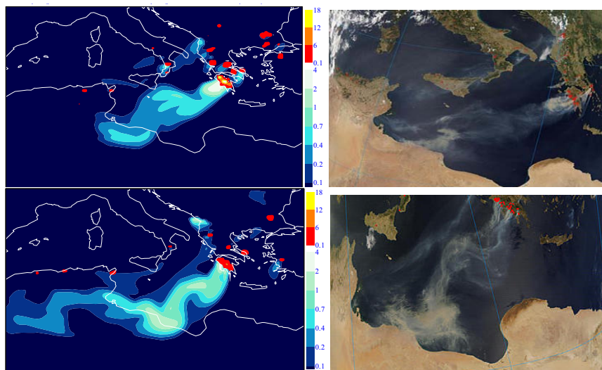
Figure 5.47: Modelled organic matter plus black carbon AOD [-] (left, blue) and MODIS visual images (right) for an Aqua overpass on 25 August, 1205UTC, (top) and a Terra overpass on 26 August, 0935UTC (bottom). Overlaid with SEVIRI FRP [W/m 2 ] interpolated to model resolution (left, orange) and MODIS hot spots in (right, red).
