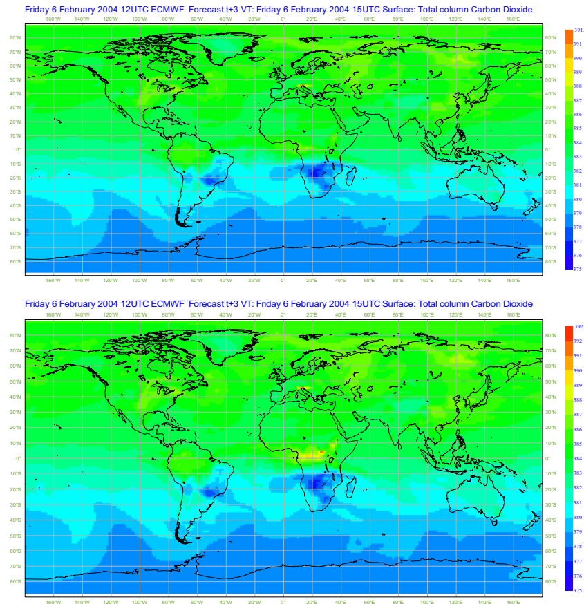
Figure 5.36: Total column CO 2 for simulation without (top) and with (bottom) fire emissions.
