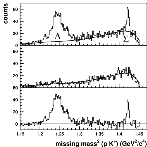
FIG. 3. Top: Spectrum of missing mass squared for the reaction pp \rightarrow pK^+X at Q = 12.9 MeV. The solid line indicates the smoothed background derived by projecting bands above and below the K^+ band of Fig. 1. Center: Background spectrum extracted as described in the text with the smoothed solid line. Bottom: Spectrum after background subtraction. Similar spectra for measurements close to the \Lambda threshold can be seen in Ref. [16].
