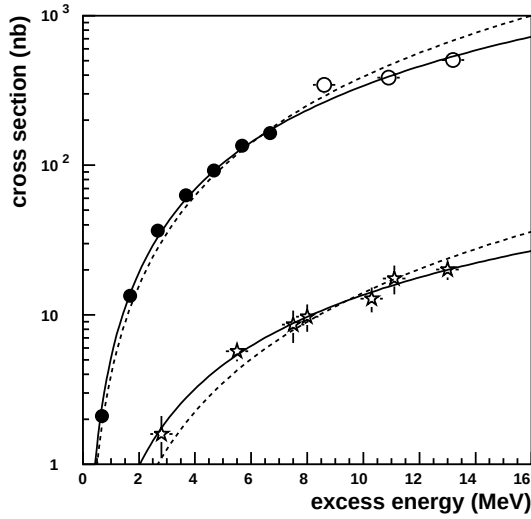
FIG. 4. Cross sections for the reactions pp \rightarrow pK^+\Lambda (circles) and pp \rightarrow pK^+\Sigma^0 (stars). Filled circles represent data published in [16]. The curves represent phase-space fits with proton-hyperon FSI (solid curve) and without (dashed line); the latter corresponds to \epsilon \rightarrow \infty in Eq. (2).
