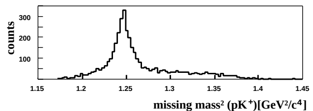
FIG. 2. Monte Carlo events for the pp \rightarrow pK\Lambda reaction at Q = 13 MeV above the \Sigma^0 threshold, analyzed similarly to the experimental data. See text for discussion.
