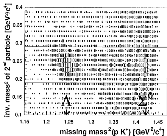
FIG. 1. Square of the mass of the second particle versus square of the missing mass, after identification of the first particle as being a proton. Data shown are at an excitation energy of Q_{\Sigma^0} = 12.9 MeV. The horizontal solid lines determine the \pm 3\sigma limits of the assumed K^+ mass distribution.
