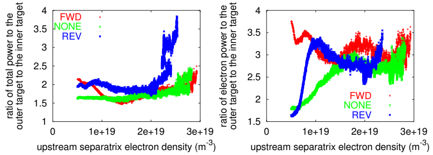
Figure 6: Ratio of total (left) and electron (right) power to the outer target to the inner target for the cases in figure 5.
