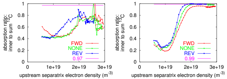
Figure 7: Absorption ratio for ^{12}\text{C} (left) and ^{13}\text{C} (right) for the inner target to sum of both targets for the cases in figure 5.
