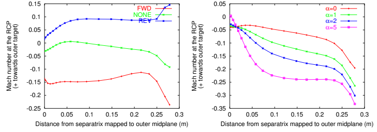
Figure 4: Left: Predicted Mach number at the position of the JET reciprocating probe position for forward, no and reversed drift SOLPS simulations with D + {}^{12}C + {}^{13}C + He . Right: Effect of transport ballooning on the predicted Mach numbers at the JET reciprocating probe position for cases without drifts but differing amounts of transport ballooning. (Compare to [15], figure 6.)
