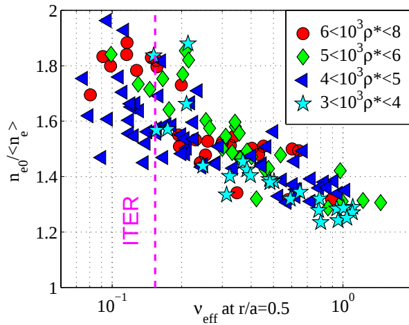
Fig. 3 Peaking factor in H-mode versus v_{eff} resolved by classes of \rho^* evaluated at r/a=0.5 .
