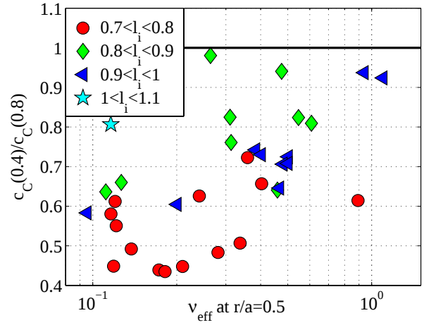
Fig. 11 Ratio of carbon concentrations at r/a=0.4 and 0.8 as function of \nu_{eff} in H-modes.
