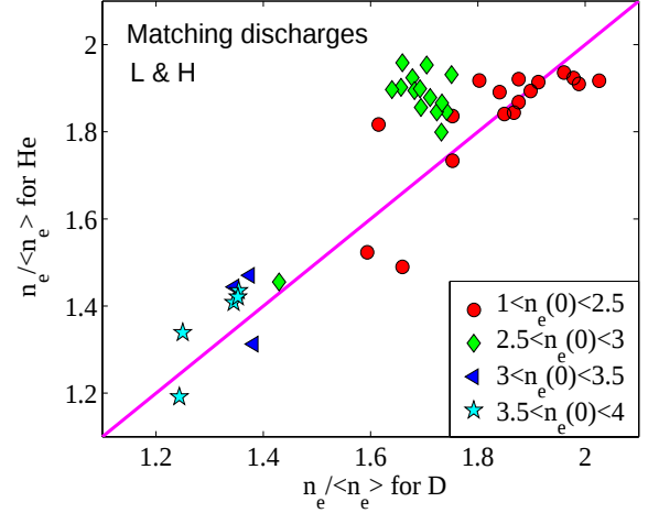
Fig. 6 Comparison of peaking factors in deuterium plasmas with their counterparts in He.
