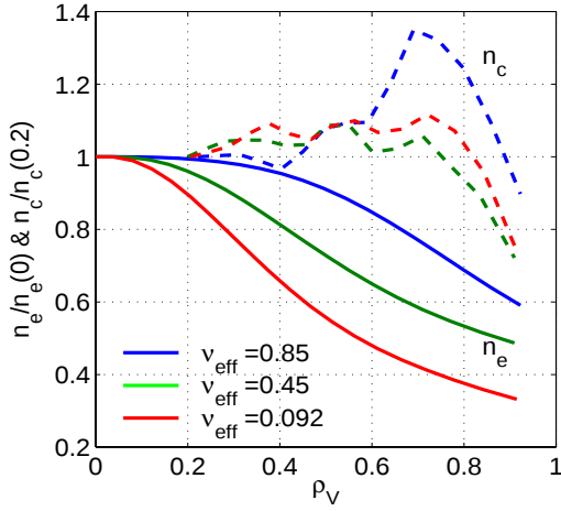
Fig. 10 Normalised H-mode electron (—) and carbon impurity density (---) profiles for three different \nu_{eff} and q_{95} \sim 3 .
