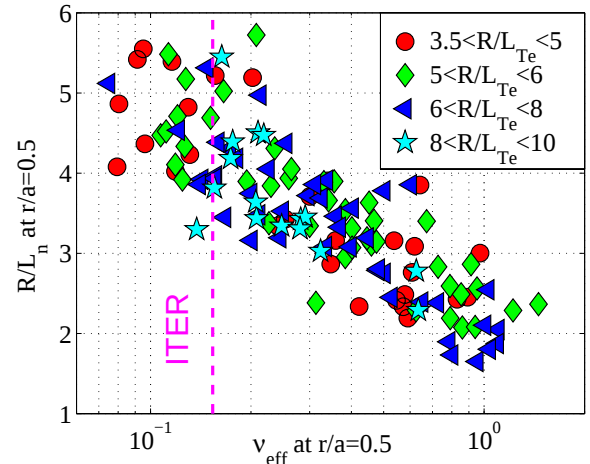
Fig. 4 Normalised electron density gradient in H-mode at r/a=0.5 versus v_{eff} , resolved by classes of electron temperature gradient.
