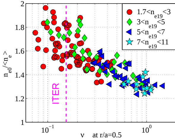
Fig. 5 As fig. 3, resolved by line average density.
