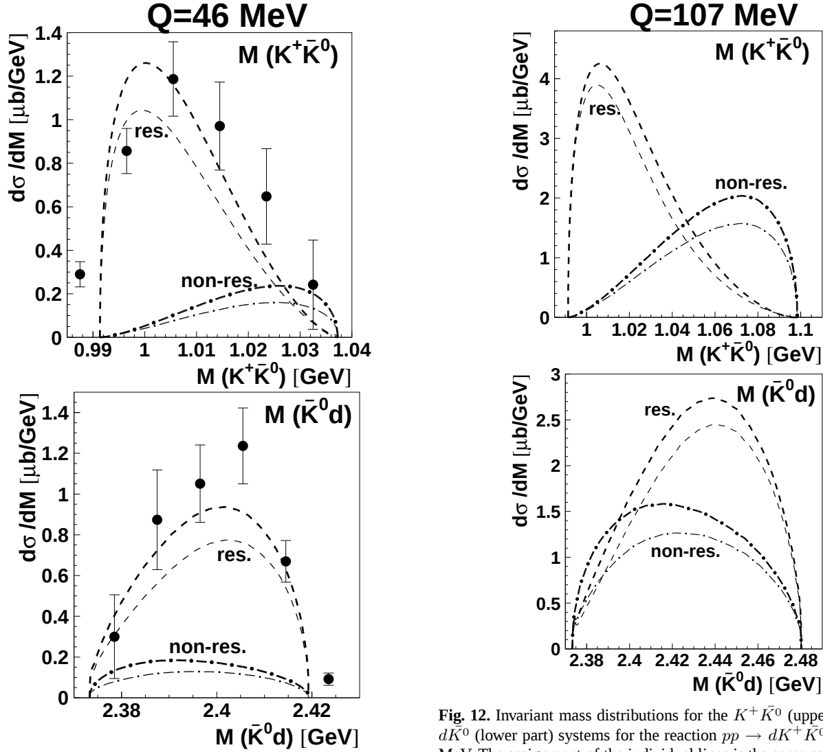
Fig. 11. Invariant mass distributions for the K^+\bar{K}^0 (upper part) and d\bar{K}^0 (lower part) systems for the reaction pp \rightarrow dK^+\bar{K}^0 at Q=46 MeV. The dashed (dash-dotted) lines are calculated for the resonance (non-resonance) contributions. The bold (thin) curves describe the contributions without (with) the FSI included. The experimental data are taken from Ref. [26].
