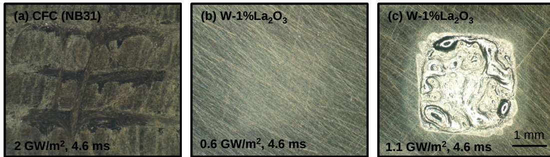
Fig.5, Microstructures of loaded surfaces. (a) CFC, 2 GW/m 2 , 4.6 ms, (b) W-1%La 2 O 3 , 0.6 GW/m 2 , (c) W-1%La 2 O 3 , 1.1 GW/m 2 , 4.6 ms.
