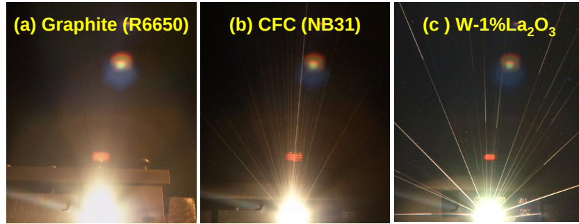
Fig.3, time integral image during thermal shock tests on (a) graphite, 2 GW/m 2 , 4.6 ms, (b) CFC, 2 GW/m 2 , 4.6ms, (c) W-1%La 2 O 3 , 1.1 GW/m 2 , 4.6 ms.
