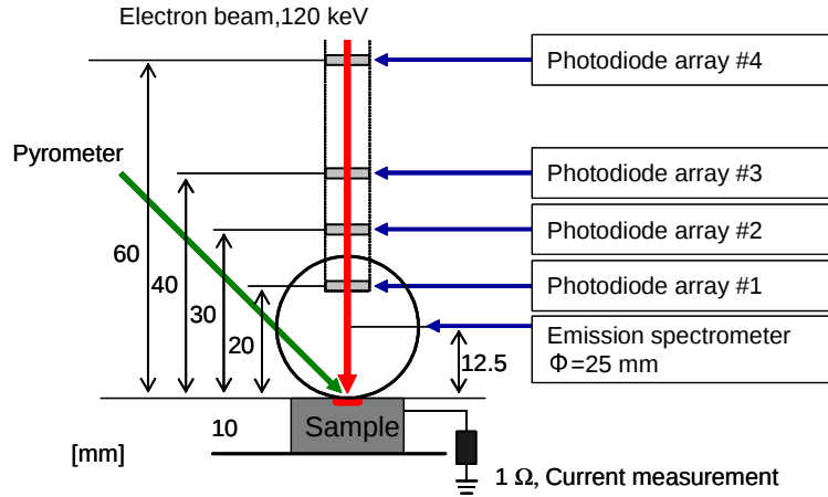
Fig. 2, Observing volumes of optical diagnostics in JUDITH.
