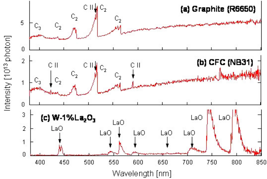
Fig.6, Spectra during thermal shock tests on (a) graphite, 2 GW/m 2 , 4.6 ms, (b) CFC, 2 GW/m 2 , 4.6ms, (c) W-1%La 2 O 3 , 0.6 GW/m 2 , 4.6 ms.
