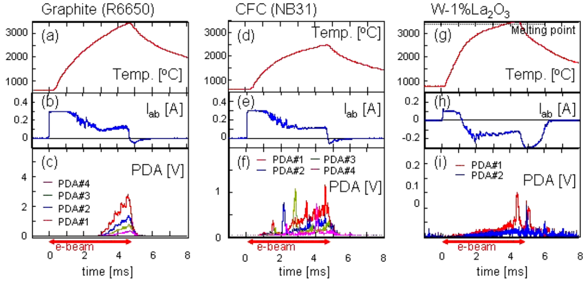
Fig.4, time evolution of surface temperatures (Temp.), absorbed currents (I ab ), PDA signals during thermal shock tests on (a) - (c) graphite, 2 GW/m 2 , 4.6 ms, (d) - (f) CFC, 2 GW/m 2 , 4.6 ms, (g) - (i) W-1%La 2 O 3 , 1.1 GW/m 2 , 4.6 ms.
