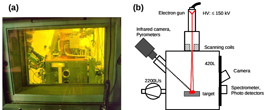
Fig. 1 Electron beam facility, JUDITH, (a) view from the outside the hot cell, (b) the schematic drawing.
