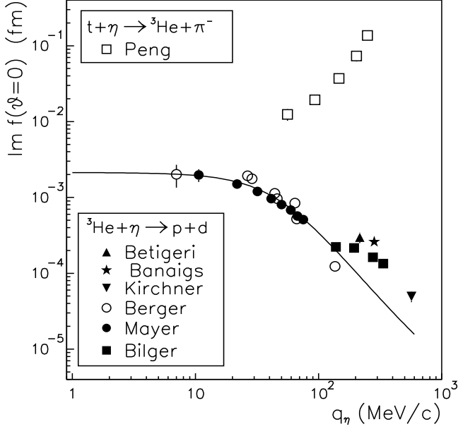
Fig. 6. Bounds on the imaginary part of the \eta - ^3\text{He} forward scattering amplitude extracted from experimental results available for the p+d \rightarrow ^3\text{He}+\eta [23,24,26,27,28,29] and \pi^- + ^3\text{He} \rightarrow t+\eta [37,38] reactions. The solid line shows our estimate based on an overall fit to low energy p+d \rightarrow ^3\text{He}+\eta data.
