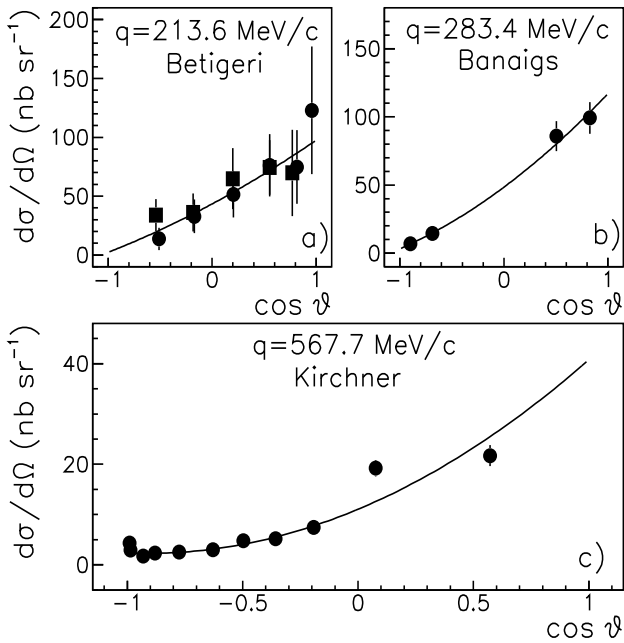
Fig. 8. Angular spectra of \eta -mesons produced in the reaction p+d \rightarrow ^3\text{He}+\eta at different final momenta q . The data are from Refs. [24,28,29]. The different symbols in (a) show results obtained with different analyzing criteria [28]. The solid lines indicate our fit.
