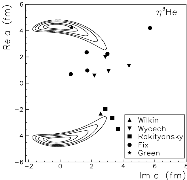
Fig. 5. Real versus imaginary part of the \eta^3\text{He} scattering length. The solid contour lines show the result of our fit to the combined data of Mayer et al. [26] and Berger et al. [23] for \chi^2+0.5 , \chi^2+1 and \chi^2+4 confidence levels, respectively. The symbols show results of various model calculations, taken from Refs. [5] (inverse triangles), [8] (squares), [9] (circles), [10] (triangle) and [11] (star).
