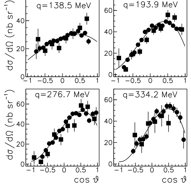
Fig. 7. Angular spectra of \eta -mesons produced in p+d \rightarrow ^3\text{He}+\eta reaction at different final momenta q . The data are from Ref. [27] where different symbols show results obtained with different analyzing criteria. The solid lines indicate the fit given in Ref. [27].
