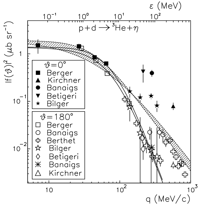
Fig. 1. Spin averaged p+d \rightarrow ^3\text{He}+\eta transition amplitude for forward (solid symbols) and backward (open symbols) \eta -meson production as a function of the final momentum q in the c.m. system (lower axis) or excess energy \epsilon (upper axis). The experiments are taken from Refs. [23,24,25]. In some cases [24,27,28,29] extrapolated results from a fit to the measured \eta -meson angular spectra are shown, cf. text. The solid lines are the fits of Ref. [23] to their p+d \rightarrow ^3\text{He}+\eta data by Eq. (9) for \vartheta=0^\circ and \vartheta=180^\circ . The shaded area indicates results based on the correlation Eq. (10) reported in Ref. [10] for the extreme limits given by \Re a=0 and \Im a=0 . Here |f|^2 was obtained by using Eq. (6).
