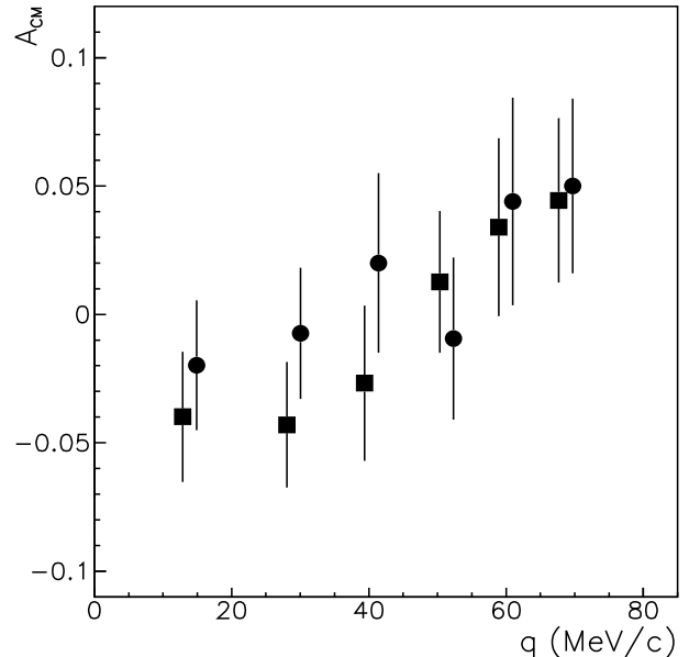
Fig. 2. Data on the \eta -meson forward-backward asymmetry A_{\text{cm}} as a function of final momentum q from Ref. [26]. The different symbols show the experimental results obtained for different analyzing criteria [26].
