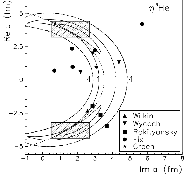
Fig. 4. Real versus imaginary part of the \eta^3\text{He} scattering length. The shaded boxes indicate the value given by Mayer et al. [26]. The solid contour lines show the result of our fit to the data of Mayer et al. [26] for \chi^2+0.5 , \chi^2+1 and \chi^2+4 confidence levels, respectively. The dashed line is the parameterization of Eq. (10) from Ref. [10]. The symbols show results of various model calculations, taken from Refs. [5] (inverse triangles), [8] (squares), [9] (circles), [10] (triangle) and [11] (star).
