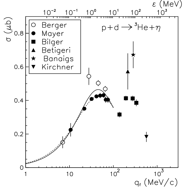
Fig. 9. The p+d \rightarrow ^3\text{He}+\eta total reaction cross section as a function of the final momentum q in the c.m. system (lower axis) or excess energy \epsilon (upper axis). The data are from Refs. [23, 24,26,27,28,29]. The solid line is our overall fit by Eq. (5) to low energy data published by Mayer et al. [26] and Berger et al. [23], while the dashed line shows our fit to the data from Mayer et al. [26] alone.
