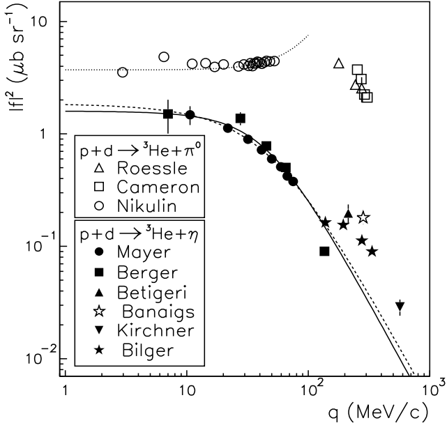
Fig. 3. Spin and angle averaged transition amplitudes |f|^2 extracted from p+d\rightarrow^3\text{He}+\pi^0 [32,33,34] and p+d\rightarrow^3\text{He}+\eta [23, 24,26,27,28,29] data on total reaction cross sections as functions of the final momentum q in the c.m. system. The dotted line shows the fit to the reaction p+d\rightarrow^3\text{He}+\pi^0 from Ref. [32]. The solid line is our overall fit by Eq. (5) to low energy data published by Mayer et al. [26] and Berger et al. [23], while the dashed line shows our fit to the data from Mayer et al. [26] alone.
