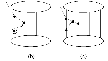
FIG. 6. NNLO diagrams with CSB stemming from soft photons.
