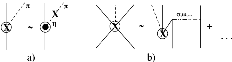
FIG. 7. Resonance saturation for (a) the CSB \pi NN vertex modeled here by \pi - \eta mixing and (b) the CSB four-nucleon operators. The ellipsis indicate that additional short-range mechanisms are to be included, as discussed in the text.
