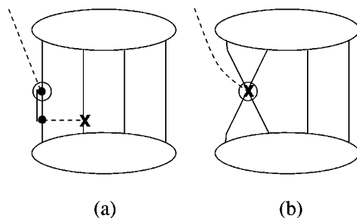
FIG. 4. Some typical higher-order diagrams with strong CSB. A double line represents a \Delta isobar. Diagram (a) appears at N^3\text{LO} whereas diagram (b) is a N^4\text{LO} contribution.
