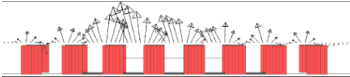
Figure 4: E (V/m) vector at a given (x, z) position in the case of a step plasma model, with magnetic shielding on the screen blades.
