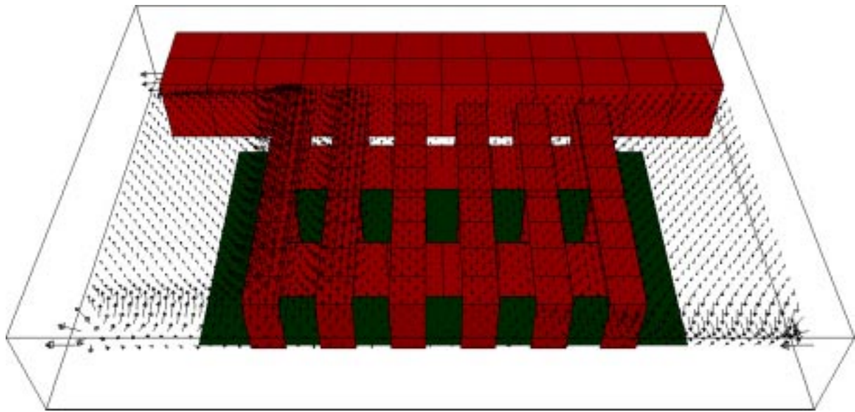
Figure 3: 3D vector map of the electric field at a fixed radial position. Case of a simplified two-strap antenna with finite screen; no magnetic shielding. Front bumper not shown.
