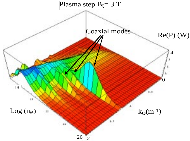
Figure 2: Radiated power mapping versus density and frequency on the fast wave in the case of a plasma step mode and a finite screen (transparency = 0.5)
