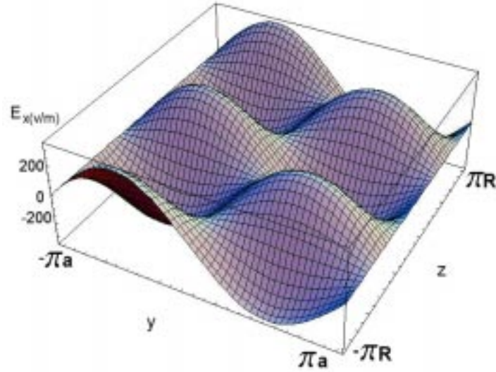
Figure 1: E_x (V/m) component of the electric field on a torus when a coaxial mode is excited.
