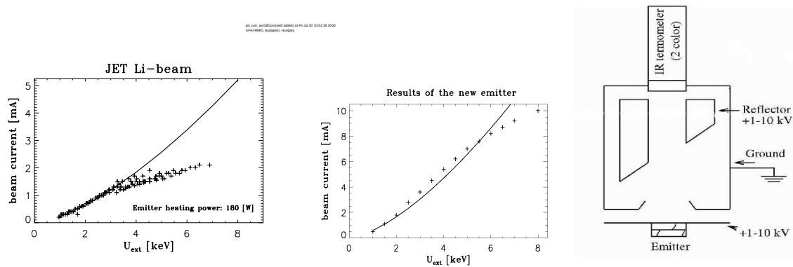
Figure 3: Beam current vs. extraction voltage and the fitted Child-Langmuir law (left). Beam current vs. extraction voltage for the new emitter (middle). Experimental setup of the testing geometry (right).
