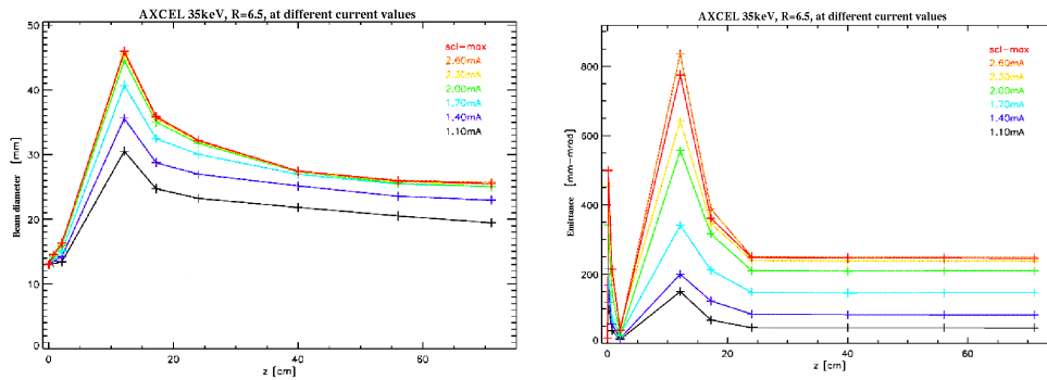
Figure 4: Beam diameter along the z-axis at different current values (left). Beam emittance at the z-axis at different current values. (right).
