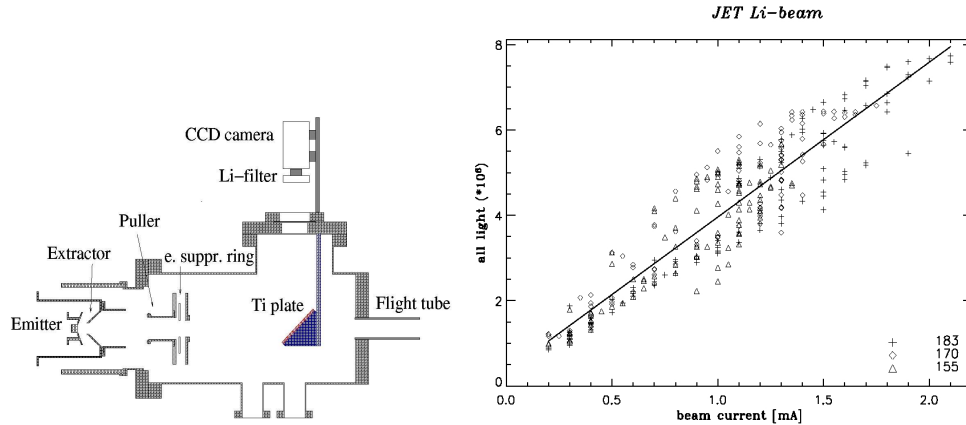
Figure 1: Experimental setup (left). Total detected light vs beam current(right).
