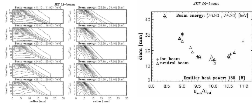
Figure 2: Beam profile plotted as a function of voltage ratio (left). Beam diameter vs. voltage ratio (right).
