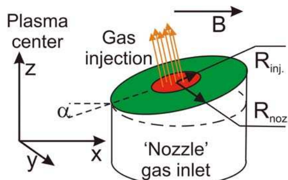
Fig. 1. Scheme of the ‘nozzle’ gas inlet geometry. \alpha - inclination angle, R_{noz.} – radius of the nozzle, R_{inj.} – radius of the injection zone, B – toroidal magnetic field.
