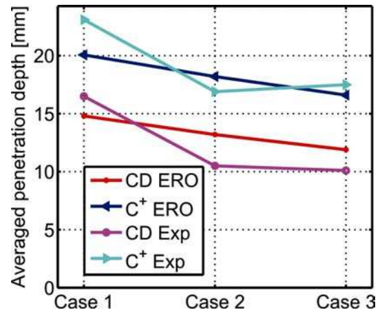
Fig. 5. Averaged penetration depth in dependence on plasma conditions.
