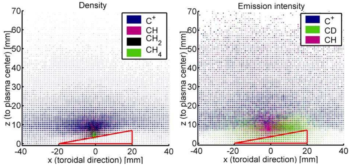
Fig. 2. Distribution of CH_4 and decay products: density (left) and light emission (right) in the observation volume (side view, 20mm nozzle radius, \alpha=10^\circ ).
