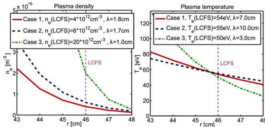
Fig. 3. 3 cases of plasma density (left) and temperature (right) in dependence of tokamak minor radius r .
