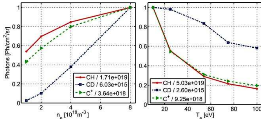
Fig. 4. Total emission of CH, CD and C + in dependence on the value of n_e (left) and T_e (right) at LCFS.
