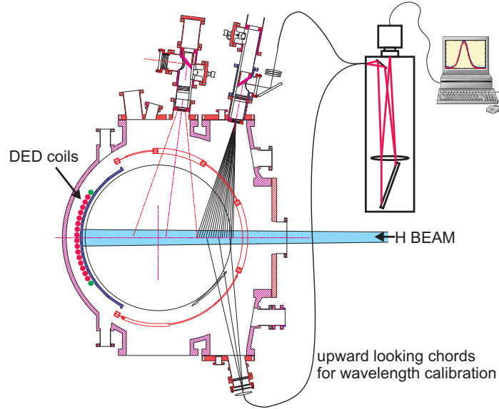
Figure 1: Set-up of the poloidal rotation measurement at the diagnostic hydrogen beam.
