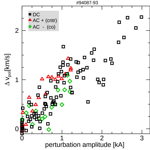
Figure 3: Change of poloidal rotation with increasing ergodization strength, represented by the DED current
