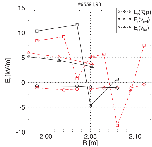
Figure 5: Contributions to the radial electric field according to equ. 1; - - DED shot; — reference shot
