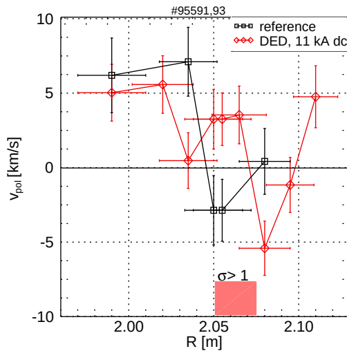
Figure 4: Poloidal rotation profiles during DED phase and a reference. The location of \sigma > 1 is calculated by field line mapping.
