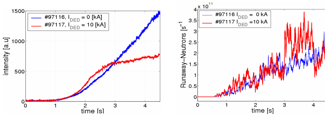
Fig. 2: Development of two runaway discharges, the blue curves show the reference case without DED and the red ones with DED (3 s to 4 s) in the m/n = 12/4 base mode. Synchrotron radiation intensity (left subfigure) represents the runaways in the discharge and the neutron signal (right) the runaway loss rate.
