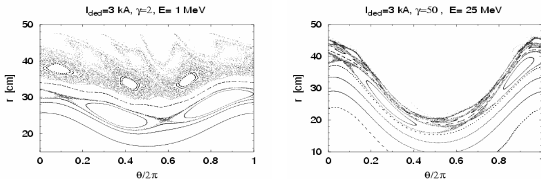
Fig.1: Poincaré plots for runaway electrons of 1 MeV (left subfigure) and 25 MeV energy for the DED base mode m/n = 3/1 .
