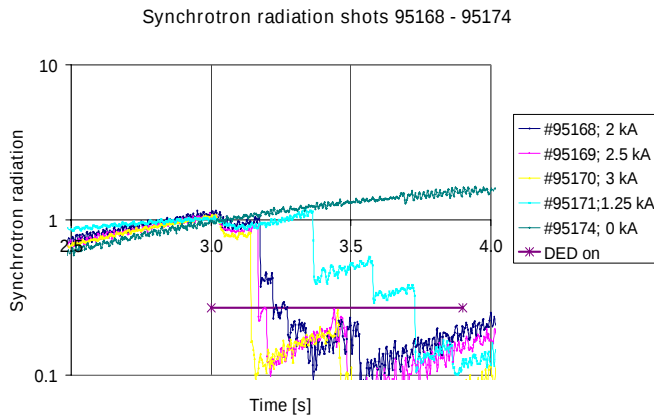
Fig. 3: Development of the synchrotron radiation for the m/n=3/1 base mode of the DED.
