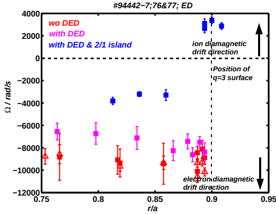
Figure 1: Turbulence rotation estimated in 3/1 configuration.
