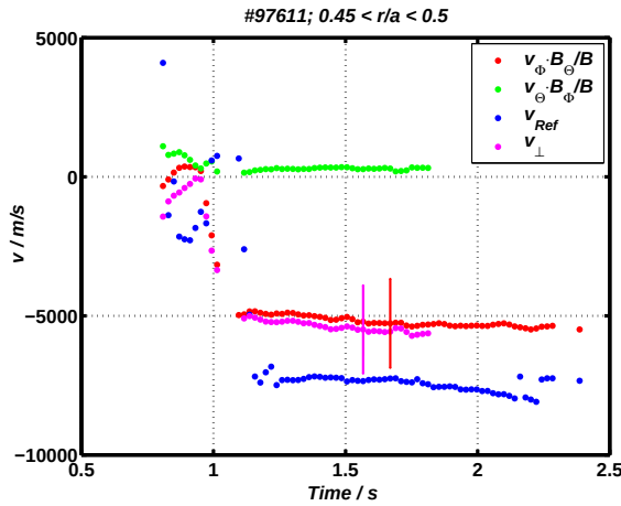
Figure 3: Calculated velocity components according eq. 1 and comparison to v_{Ref} for a plasma with P = 1.2 MW counter neutral beam injection and P \approx 300 kW co-injection.
