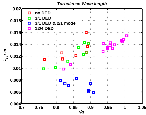
Figure 5: Estimated \langle \lambda_\Theta \rangle from autocorrelation function. The locked 2/1 mode during 3/1-configuration yields to a reduction of \langle \lambda_\Theta \rangle which is an indication of a reduced transport
