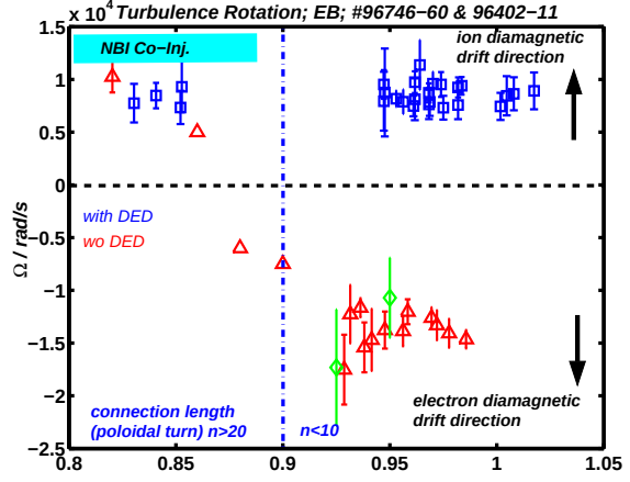
Figure 2: Turbulence rotation in 12/4 configuration. In addition \Omega_\Theta estimated from Doppler shifted carbon ions is shown in green
