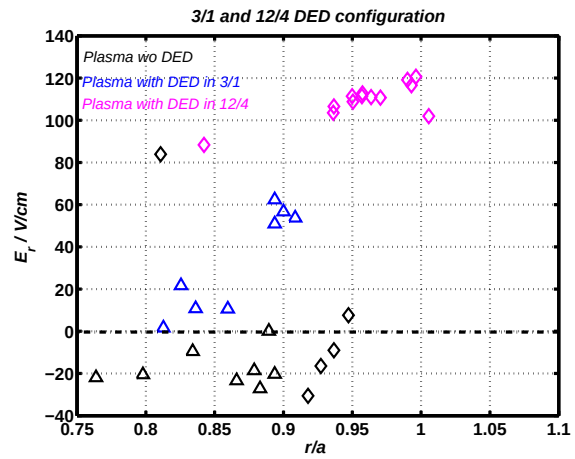
Figure 4: Estimation of E_r in plasmas with 12/4– (diamonds) and 3/1–configuration (triangles). For comparison E_r is also estimated for both sets of plasma parameters without DED.
