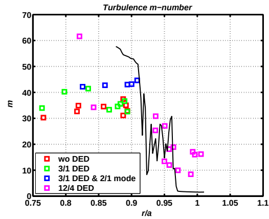
Figure 6: As expected the poloidal mode number during 12/4 operation drops significantly in the divertor region. In 3/1-configuration the mode number is not changed.
