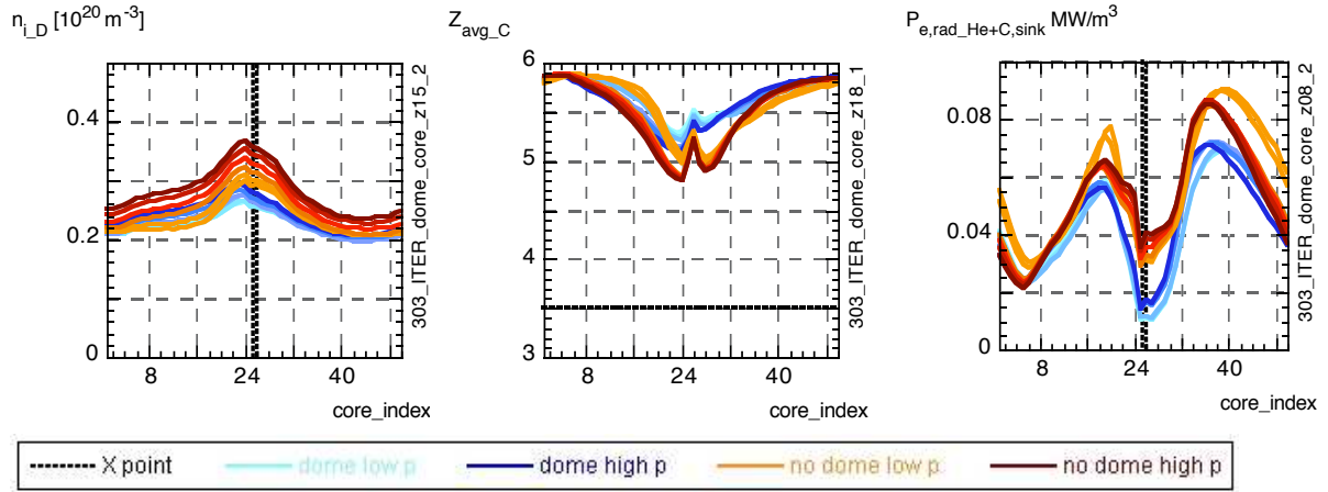
Fig. 3. Poloidal variation of a) deuterium density, b) average C ion charge state, c) line radiation per unit volume just inside the separatrix, Ordinate is poloidal coordinate counter-clockwise, starting from the top, X-point at 25.5; blue with dome, red without dome, darker shades are higher p_{DT} .
