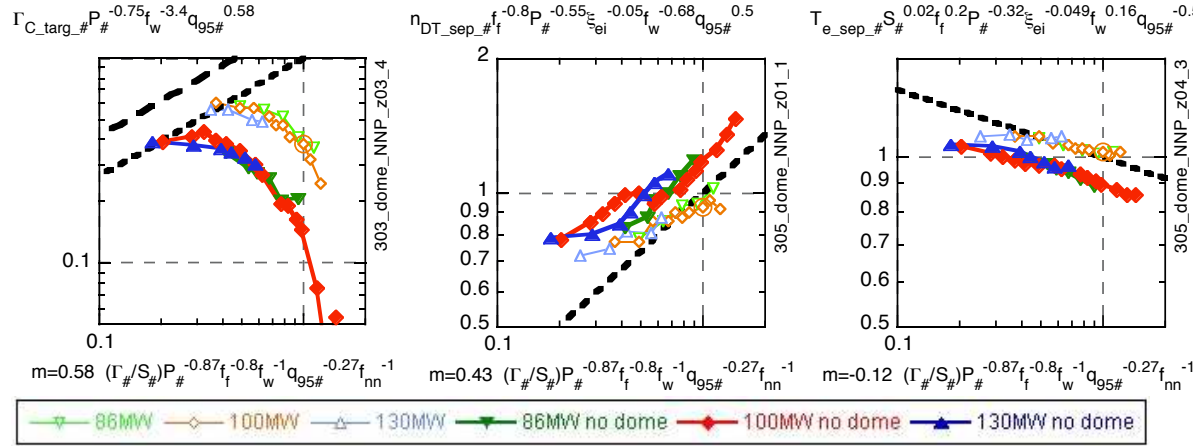
Fig. 2. a) Normalised net target erosion, b) separatrix DT density and c) separatrix electron temperature vs normalised p_{DT} ; for cases with dome and without (indicated as such).
