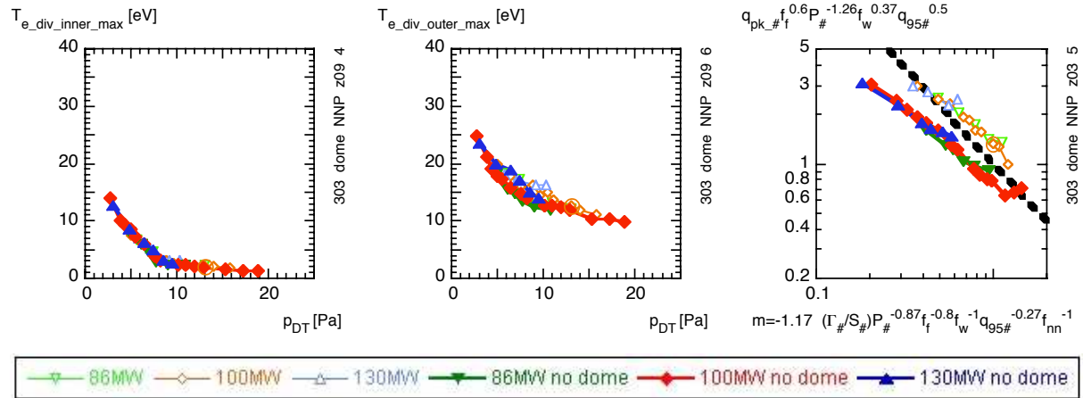
Fig. 1. Maximum electron temperatures at inner and outer targets vs. p_{DT} , and normalised peak power loading of the outer divertor vs. normalised p_{DT} . See [3] for the normalisation.
