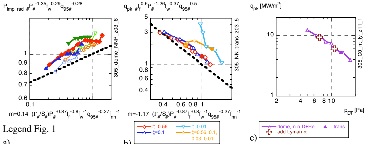
Fig. 4. a) normalised impurity radiation vs normalised p_{DT} , ; normalised peak power load vs b) norm. p_{DT} for variation of transparency and vs. c) p_{DT} for radiation transport effect (see text).
