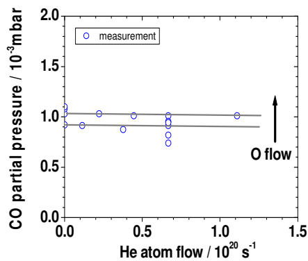
Fig 2: CO partial pressure at different O 2 injection rates depending on the He injection rate.
