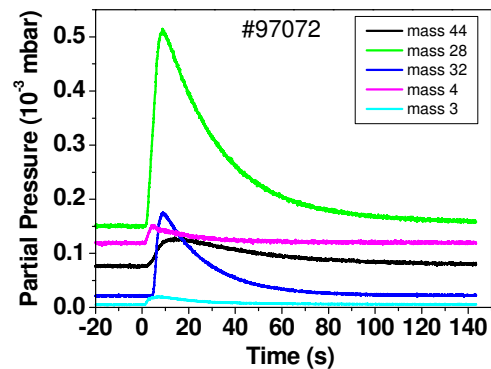
Fig 5: temporal behaviour of CO, CO_2 , O_2 and HD partial pressure during and after ICRF pulse. The ICRF pulse lasted from 1-2.7 sec and oxygen was injected at 1.1.-4 sec with rate of 3 \cdot 10^{20}/\text{sec} .
