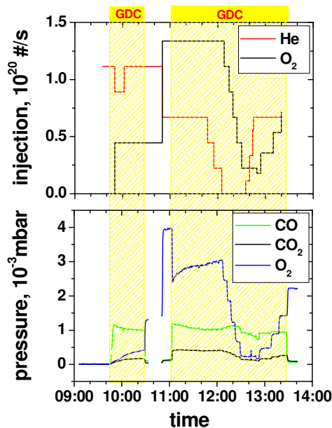
Fig 1: Temporal evolution of the O 2 and He injection rates (upper) and the partial pressures of CO, CO 2 and O 2 . The shadowed areas indicate GDC on/off.
