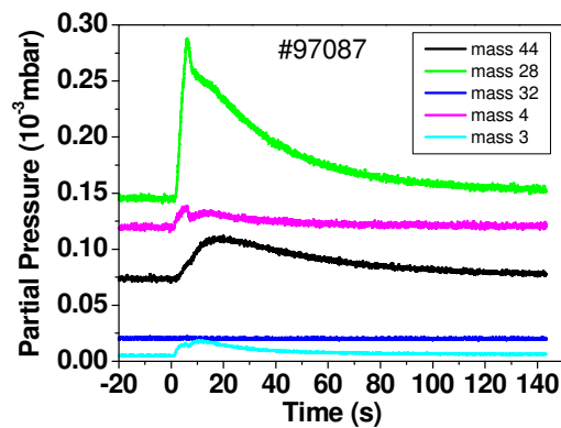
Fig 4: temporal behaviour of CO, CO_2 , O_2 and HD partial pressure during and after ICRF pulse. The ICRF pulse lasted from 1-3.9 sec and oxygen was injected at 1.1.-4 sec with rate of 2.1 \cdot 10^{20}/\text{sec} .
