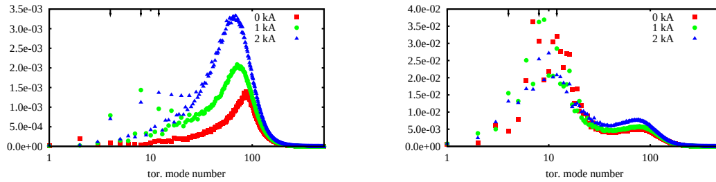
Figure 5: Fourier amplitude plot of the turbulent E \times B flux \langle \Gamma_n \rangle_{xt} vs toroidal mode number n for \nu_B=0.04 (left) and \nu_B=1.48 (right)
