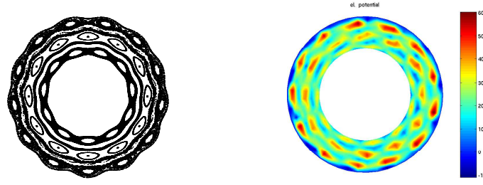
Figure 3: Poincaré-plot of the island structure for an coil current of I_D=0.3 kA (left) and poloidal pattern of the static piece of the electric potential for a coil current of I_D=1 kA (right)
