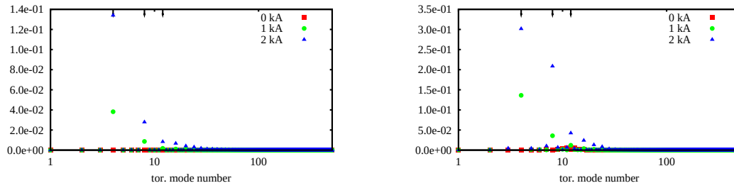
Figure 4: Fourier amplitude plot of the static E \times B flux \langle \Gamma_n \rangle_{xt} vs toroidal mode number n for \nu_B=0.04 (left) and \nu_B=1.48 (right)
