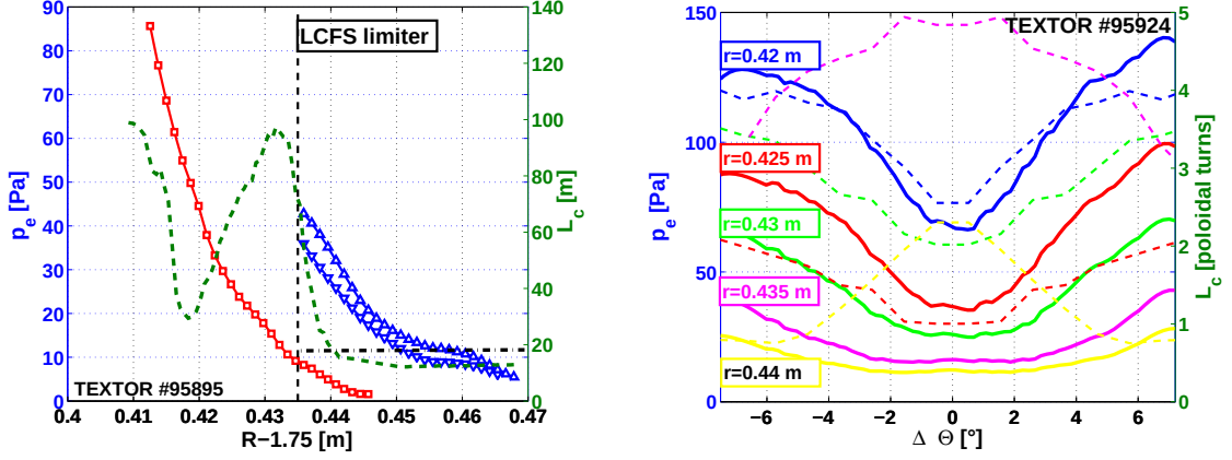
(a) Profiles p_e(r) with (red line with squares) and without (blue lines with triangles) DED (b) p_e(\Theta) (solid lines/left abscissa) and L_c(\Theta) (dashed lines/right abscissa) during sweep
