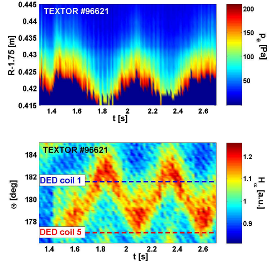
Figure 3: H_\alpha(\Theta, t) pattern on DED target and p_e(\Theta, t) at LFS follow sweep of DED currents
