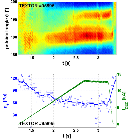
Figure 1: Upper subplot: time evolution of H_\alpha in the region of one paired footprint on DED target
