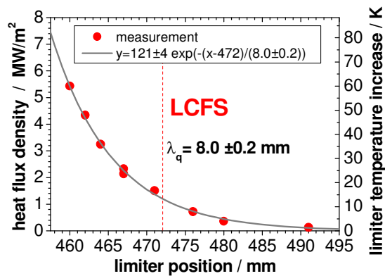
Fig.1 Peak heat flux density on the tungsten plate surface measured by thermocouples
