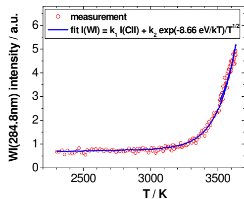
Fig.6 Tungsten flux versus temperature
