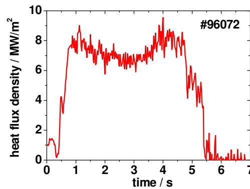
Fig.2 Heat flux density derived from pyrometer at r=46 cm
