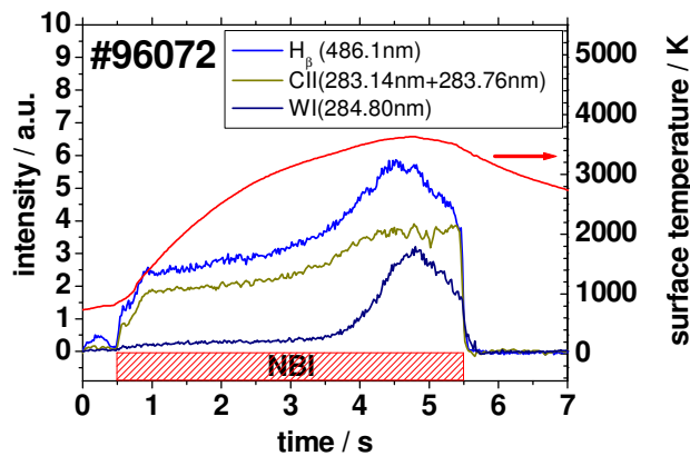
Fig.5 Evolution of spectral line intensities and surface temperature
