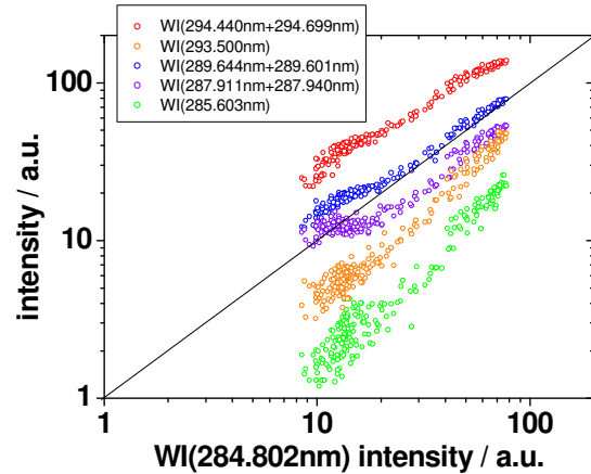
Fig.3 Spectrum measured in front of W plate Fig.4 Spectral line intensities dependences.
