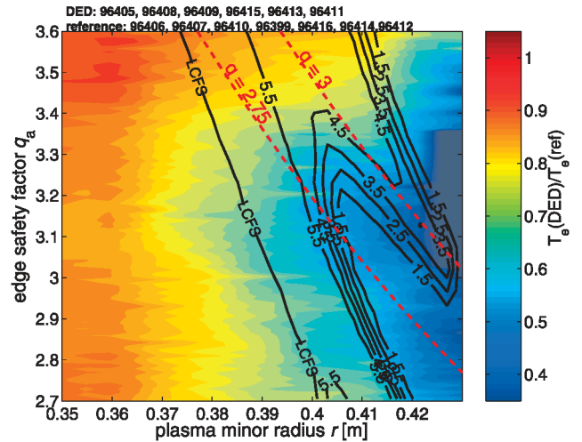
FIG. 3 (color). The contour plot of the drop in the electron temperature in the plasma edge measured by the ECE [20] as a function of the plasma minor radius (abscissa) and the value of the safety factor at the plasma edge— q_a (ordinate). The profiles obtained for the DED case were divided by the profiles measured for analogous discharge without the DED. The solid black lines represent the contour plot of the calculated connection lengths. The red dashed lines indicates the position of the q = 3 and q = 2.75 surfaces.
