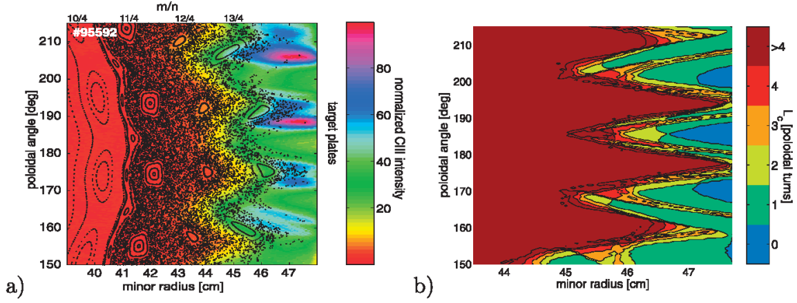
FIG. 1 (color). (a) The two-dimensional distribution of the CIII emission in the front of the DED coils for discharge #95592 overlaid with the Poincaré section visualizing the structure of the magnetic field calculated with the ATLAS code. The color bar indicates the intensity of the CIII line at 465 nm in the arbitrary units. The m/n numbers on the top of the figure indicate the island chains. (b) Corresponding laminar plot representing the contour plot of the field lines connection length calculated for the same conditions as in (a).
