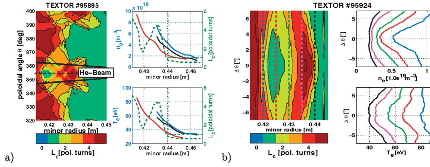
FIG. 2 (color). The influence of the laminar zone on the plasma electron temperature and density. (a) The radial profiles of the electron density (top right) and electron temperature (bottom right). The red curves present the data measured during the DED phase, the blue curves the data before the DED phase, and the black one the data after the DED phase. Green lines (right ordinate): calculated with the ATLAS-code connection lengths of the field lines for the coordinates of the measured profiles: DED case (dashed line); non-DED case (dash-dotted line). On the left, the laminar plot visualizing the magnetic-field topology during discharge #95895 is presented beam. Black lines visualize the geometry of the thermal helium beam. (b) On the right, the poloidal variation of the plasma electron density (top) and temperature (bottom) measured during the slow (1 Hz) sweep of the perturbation field. On the left, the effective laminar plot visualizing the magnetic topology. The data represent a convolution of calculated L_c values and the spatial resolution of the diagnostic. Dashed lines indicate the coordinates at which n_e and T_e profiles are measured.
