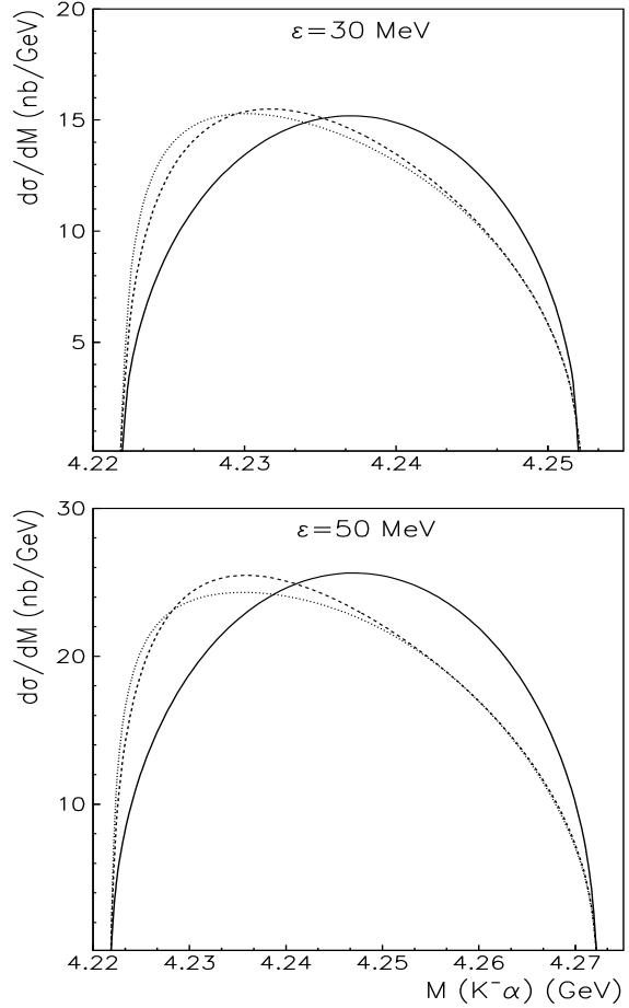
Fig. 3. The invariant K^- \alpha mass spectra produced in the dd \rightarrow \alpha K^+ K^- reaction at excess energies 30 and 50 MeV. The solid lines describe the pure phase space distribution, while the dashed and dotted lines show our calculations with K^- \alpha FSI given by parameters of Set 1 and 4, respectively.
