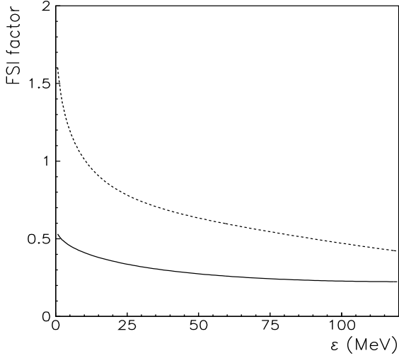
Fig. 2. The K^- \alpha FSI factor averaged over the three body phase space of the reaction dd \rightarrow \alpha K^+ K^- as a function of excess energy. The solid and dashed lines show the calculations with parameters of Set 1 and 4, respectively.
