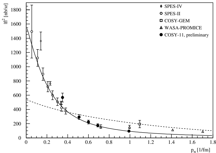
Fig. 1. Average production amplitude squared |ff|^2 as function of the cms momentum of the emitted \eta mesons for the pd \rightarrow {}^3\text{He} \eta reaction. The solid and dashed lines represent fits to the data based on a strong \eta - {}^3\text{He} FSI and a resonance model description respectively.
