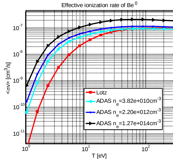
Fig.1. Old (Lotz) and new (ADAS) effective ionization rates for neutral Be used by ERO.
