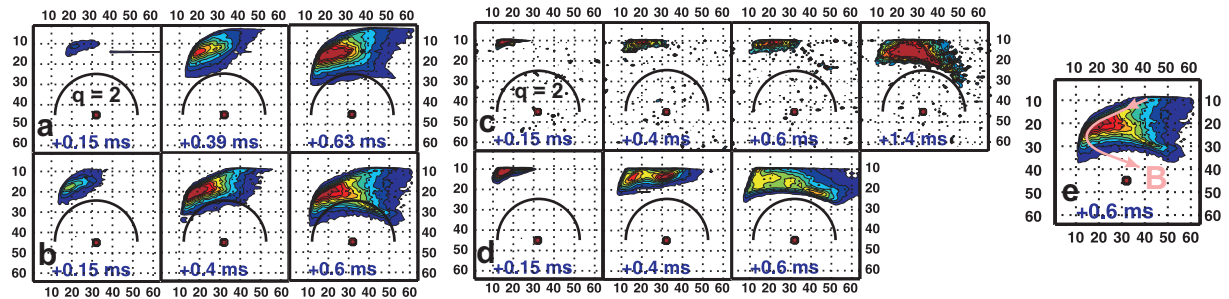
Figure 4: Contour plots of initial gas penetration into plasma. a - TEXTOR shot 99688, He 1.5 bar injection, He II filter. b - TEXTOR shot 100168, He 4.5 bar injection, He II filter. c - TEXTOR shot 100934, Ar 3 bar injection, Ar II filter. The noise is produced by RE induced neutrons or X-rays. d - TEXTOR shot 100936, D_2 + 10\% \text{ Ar} 3 bar injection, Ar II filter. For further explanations see fig. 3. e - Magnetic geometry illustrated on the last frame of sequence b . The toroidal magnetic field goes through the paper. The major axis of the tokamak is to the right.
