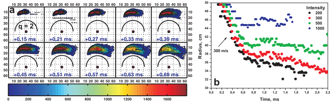
Figure 3: a - contour plots of initial gas penetration into plasma. TEXTOR shot 99685, He 1.5 bar injection, He I filter. Axes are in pixels, 1.5 cm/pix. Point at the position x = 32, y = 45 is the center of the discharge. The semicircle represents the position of the q = 2 surface. Not all frames are shown. Time is given relative to the detection of the jet at the edge of the plasma. b - the shortest distance from different intensity contours to the plasma center as a function of time.
