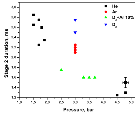
Figure 2: The duration of stage 2 for different gasses and initial pressures.
