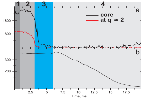
Figure 1: Time traces of the main plasma parameters for the TEXTOR shot 99685, an He injection. a - ECE measurements of the electron temperature at the q \approx 2 (red curve) and in the center (black curve), eV; b - plasma current, kA. The time is given in ms relative to mitigation valve trigger signal.
