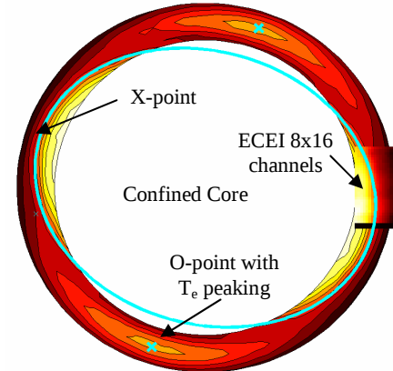
Figure 1: Poloidal reconstruction of ECRH heated island
