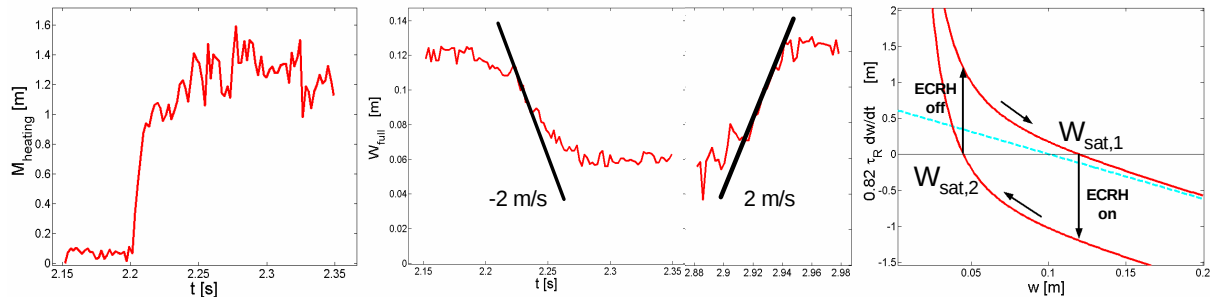
Figure 3: The suppression process: a) The heating term b) The experimentally observed growth/suppression rates c) Overview of the various terms in the modified Rutherford equation.
