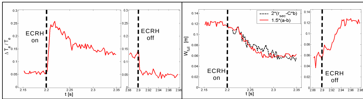
Figure 2: Typical time evolution of relative T_e peaking and island width.
