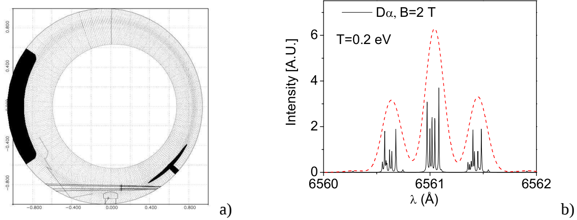
Figure 2: a) Plot of a poloidal cross section of the TEXTOR case. The bumper limiter is on the high field side (left), and the ALT limiter is on the low field side. The black solid lines figure the chords observing above the test limiter, which is positioned at r = 48 cm. b) Line shape retaining Zeeman, Stark and fine structure effects, with (dashed) and without Doppler broadening (solid).
