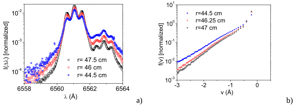
Figure 3: a) High resolution D\alpha/H\alpha spectra measured in TEXTOR. b) Simulated VDF for 3 different chords providing radial resolution.
