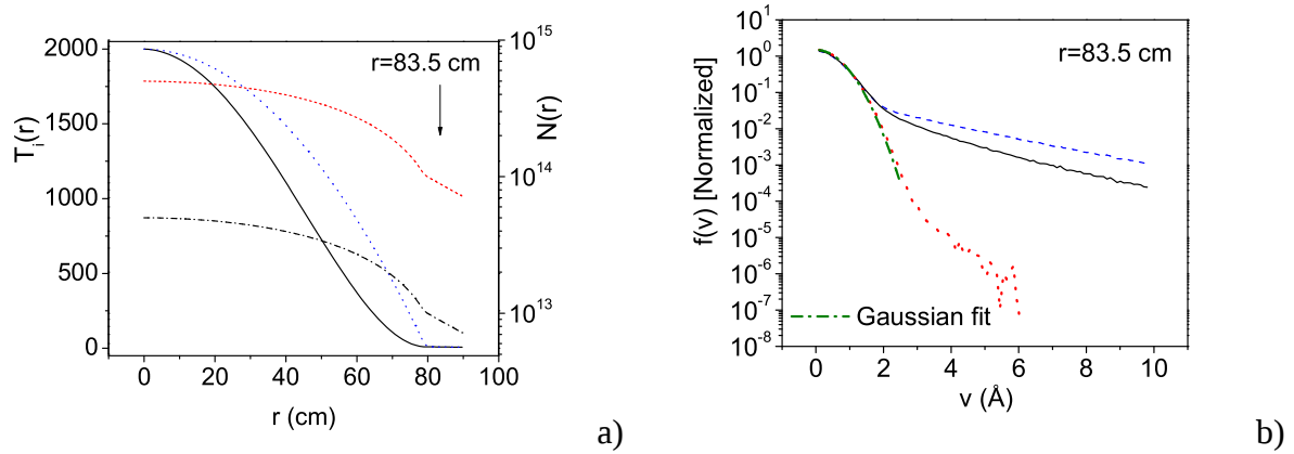
Figure 1: a) Density profiles (dashed-dotted black and short dash red, log. scale) and temperature profiles (solid black and dotted blue) used in the simulations. b) Calculated VDF at r = 83.5 cm. The velocity is expressed in terms of the equivalent Doppler shift (Å) for the D\alpha line. The green dashed-dotted line is a Gaussian fit, giving a temperature very close to the local T_i .
