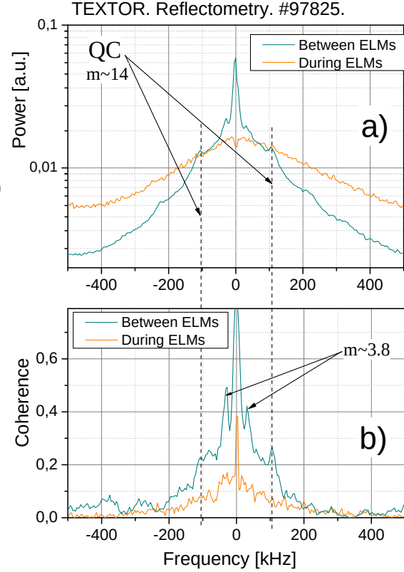
Figure 4: Turbulence power spectra (a) and coherence (b) obtained between and during ELMs (conditional averaging over \approx 1 s is used) show rather different turbulence properties.
