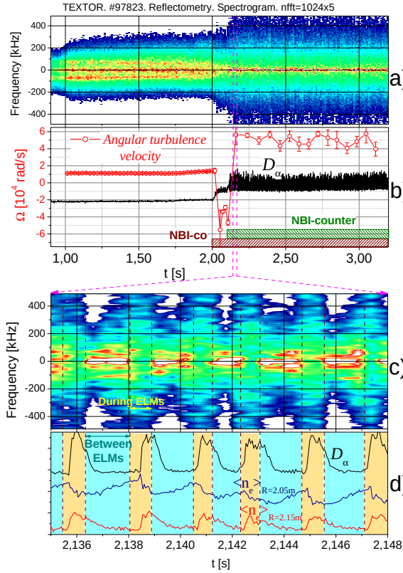
Figure 3: Turbulence spectrum evolution (a) and time traces of the turbulence rotation and D_\alpha signal (b). The detailed phasing between turbulence spectrum (c), D_\alpha and periphery density behavior (d).
