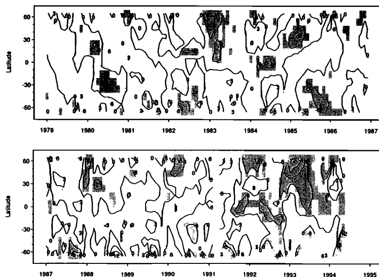
Figure 14. Contour plots of total ozone residuals as a function of latitude and time from the statistical fit to the SBUV(2) satellite total ozone data from January 1979 to May 1991. The fitted model was extrapolated through May 1994 to calculate the residuals over the extended period January 1979 to May 1994. The total ozone data have the seasonal, trend, solar, and quasi biennial oscillation (QBO) components removed, and the resulting deviations are expressed as percentages of the mean ozone level at the beginning of the series. Contours show constant deviations at intervals of 3%, and the shaded areas indicate negative departures of at least 2%. The 1992-1993 low ozone values are prominent, as well as other periods of very low values in 1982-1983 and 1985.
