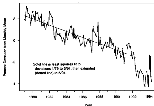
Figure 13. Total ozone (60°N–60°S) from January 1979 to May 1994 measured by SBUV/(2). The annual cycle and the effects of the solar cycle and QBO have been removed. The solid line is a simple least squares fit to the data through May 1991. The dashed line is an extrapolation through May 1994.
