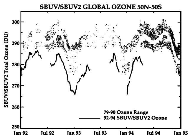
Figure 12. Total ozone (50°N–50°S) measured by SBUV/2 since January 1992 compared with the 1980s range and average from the combined SBUV/(2) record.
