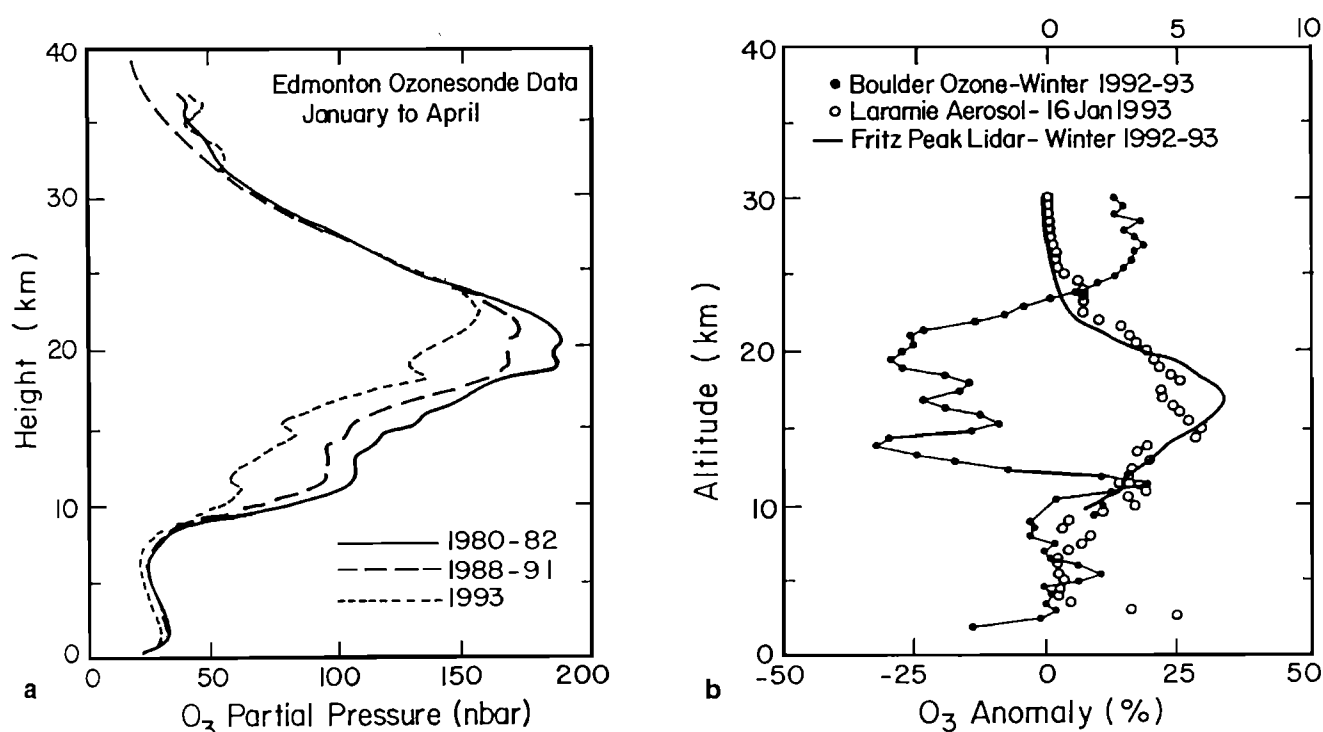
Figure 15. (a) Average ozone profiles found from ozonesonde measurements at Edmonton in spring (January to April) for 1980-1982 (46 sondes), 1988-1991 (42 sondes), and 1993 (13 sondes) [adapted from Kerr et al. , 1993]. (b) Percentage differences (bottom axis) in the ozonesonde measurements at Boulder in 1992-1993 relative to 1985-1989. Also shown are the aerosol data from the Fritz Peak lidar (bottom axis, backscatter in 10^8 \text{ ST}^{-1} \text{ m}^{-1} ) and the University of Wyoming particle counter (top axis, aerosol concentration in \text{cm}^{-3} ) for winter 1992-93 [adapted from Hofmann et al. , 1994a].
