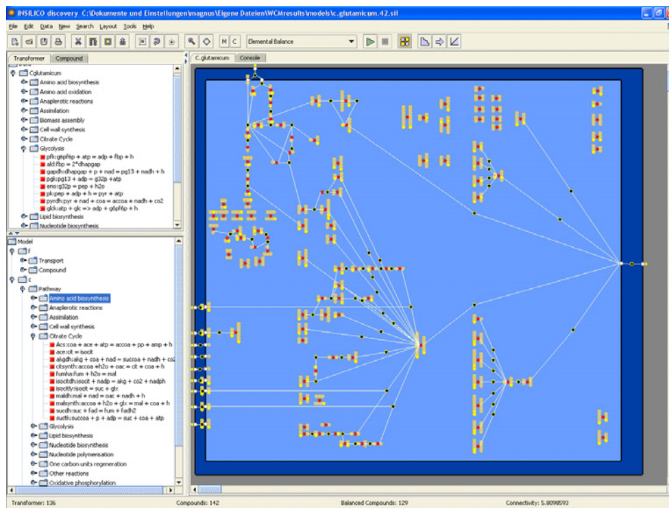
Figure 2–8: The graphical user interface of In-Silico Discovery. The model development is done directly on the GUI. The reactions can be typed in manually or can be added from a database. The panel in the upper left corner shows the list of reactions in the reaction database while the lower panel on the left hand side shows the reactions already included in the model. The main frame gives a graphical representation of the reaction network.
