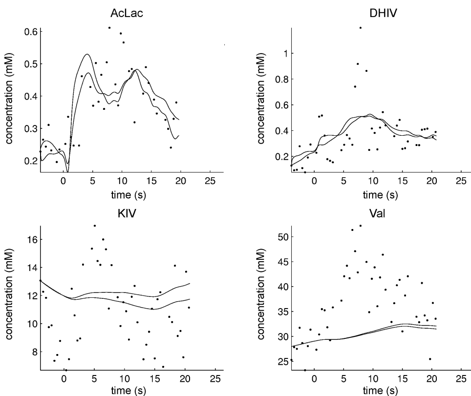
Figure 9-1: The simulated time courses of the metabolites in the valine pathway by the mechanistic model for the two best fitting parameter sets.
