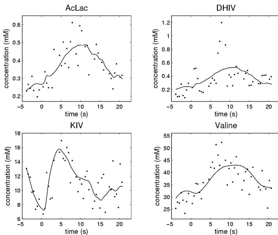
Figure 6-1: The simulation of the intracellular metabolites in the valine pathway (lines) and the measurements that were used to fit the parameters in the model (dots). The glucose stimulus was added at time 0.
