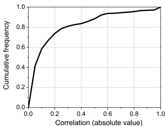
Figure 6–5: The cumulative frequency distribution of the parameter correlations. The curve is used to determine the percentage of the correlations that lie below a certain value. It can for example be seen that about 80 % of the correlations are less than 0.3 in absolute value.
