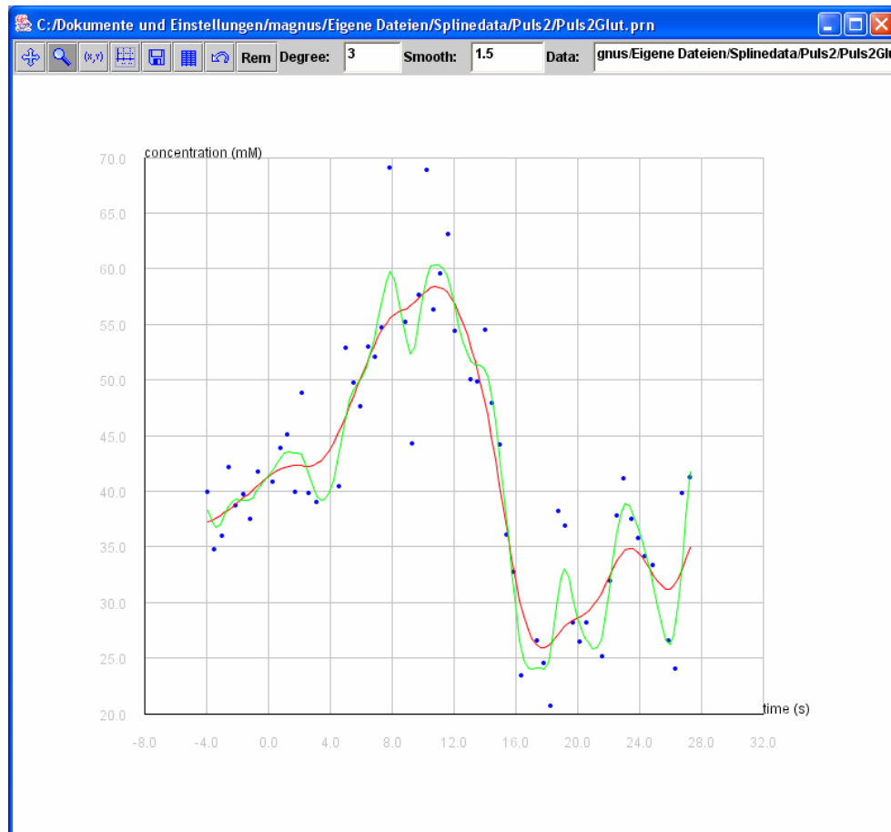
Figure 4-4: The graphical user interface of the spline program. In the field “Data” the path to the file containing the concentration data can be specified. In the text fields “Degree” and “Smooth” the degree and smoothness factor of the splines can be specified. The red line shows a spline with a large smoothing factor and the green line a spline with a smaller smoothing factor. The blue points are the concentration data from which the splines are calculated.
