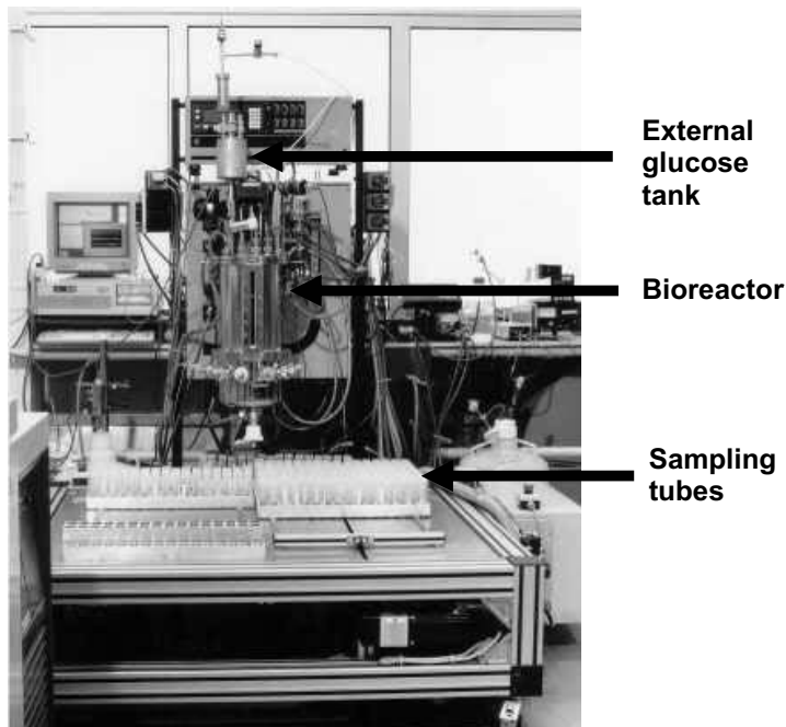
Figure 2–2: Picture of the stimulus and rapid sampling apparatus.
