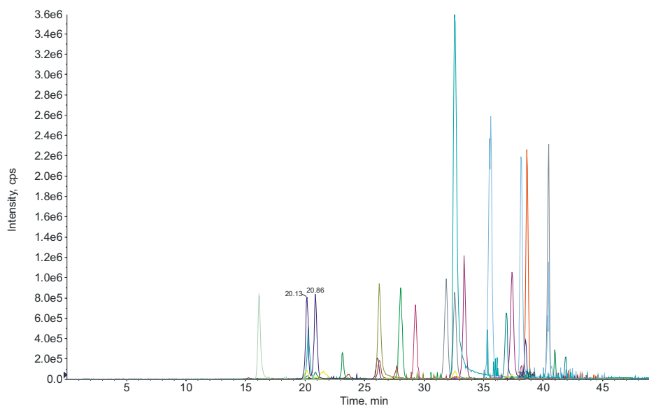
Figure 3–2: The chromatogram for the measurements on the mass spectrometer from Applied Bioscience. The peaks of the different masses are shown in different colours.
