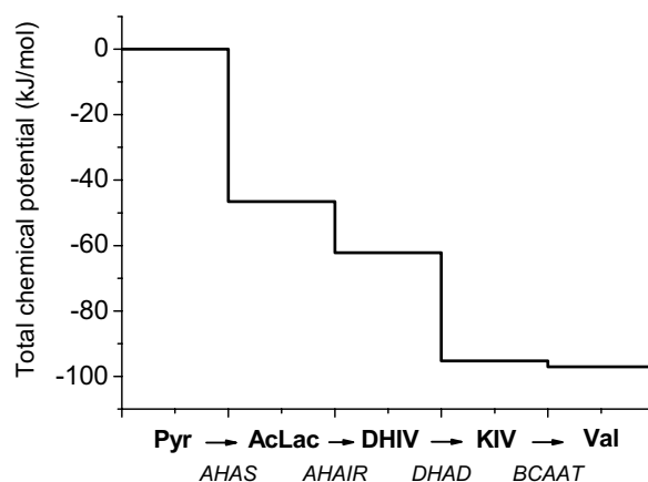
Figure 8-1: The fall of Gibbs free energy, or total chemical potential, through the valine pathway. The values on the y-axis show the total chemical potential of the metabolites participating in the reactions in the valine pathway at different stages through the reaction sequence. The total chemical potential of the metabolites before the first reaction was used as a reference point and set to 0. The diagram then displays how the chemical potential of the reactants decrease as the reaction proceed through the valine pathway. The values of the chemical potentials are given in kJ per mol of valine formed.
