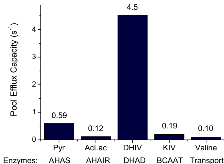
Figure 7–1: The Pool Efflux Capacities of the enzymes in the valine pathway.
