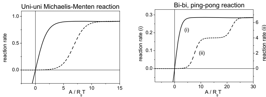
Figure 8-3: The reaction rate dependence on the affinity. Left: the uni-uni Michaelis Menten reaction according to Eq. (8-2). The full line is a reaction with A'' = 0 (i.e. K_{eq} = 1 ) and the broken line a reaction with A'' = 17.4 kJ/mol ( K_{eq} = 1000 ). In the first case the kinetic parameters and the concentration constraint were set to V_F = V_R = K_B = K_P = 10 , (x_B + x_P) = 1 . In the second case the kinetic parameters and the concentration constraint were set to V_F = K_B = K_P = 10 , V_R = 0.1 , (x_B + x_P) = 1 . This diagram was also reported by Westerhoff and van Dam (1987). Right: the bi-bi ping-pong reaction according to Eq (8-6). The full line is a reaction with A'' = 0 (as for the BCAAT reaction) and the broken line is a reaction with A'' = 53.4 kJ/mol (as for the AHAS reaction). In the first case all parameters as well as the concentration of B and P were set to 1 and the sum of x_C and x_Q was set to 2. In the second case the parameters and constraints were set to V_F = K_P = K_Q = 10 , V_R = K_{i,Q} = K_{i,B} = x_B = x_P = 1 , K_C = 0.5 and (x_B + x_Q) = 2 .
