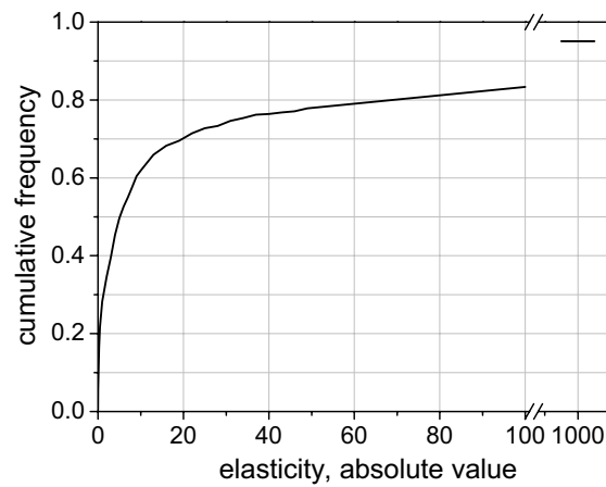
Figure 9–5: The cumulative frequency distribution of the absolute values of the elasticities in the whole cell model. The elasticities from the first of the 16 parameter sets are displayed. This set is representative of the other sets.
