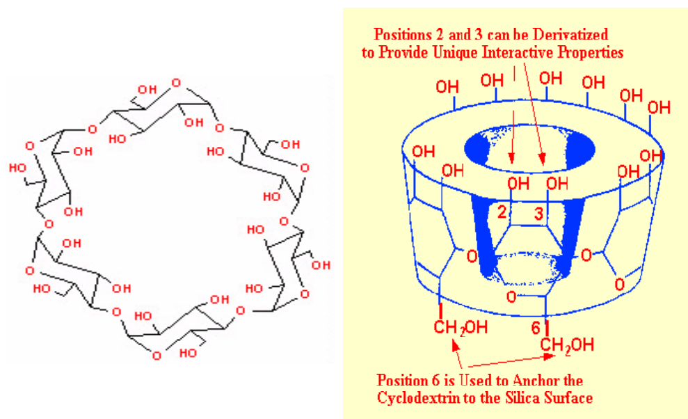
Figure 2–6: The structure of the \beta -cyclodextrin columns.
