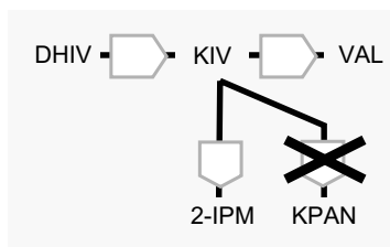
Figure 5–7: The KIV branch point. Valine is produced in one transamination step from KIV. The leucine pathway starts with the formation of 2-isopropylmalate (2-IPM) from KIV. The pantothenate pathway also bifurcates off from the KIV branchpoint with the formation of KPAn. In the investigated strain the panB gene coding for ketopantoate hydroxymethyl transferase has been deleted and the reaction forming KPAn should therefore not take place.
